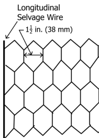
FIG. 1 Type TW—Twisted Hexagonal Mesh (Design Number 7.5 \times 0 \times 0.054 \times 0 )
