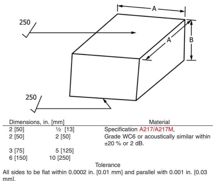
FIG. 3 Calibration Blocks
