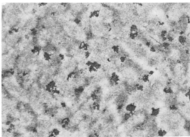
FIG. X1.4 Grade M5503, Approximately HB 229 (100x)
