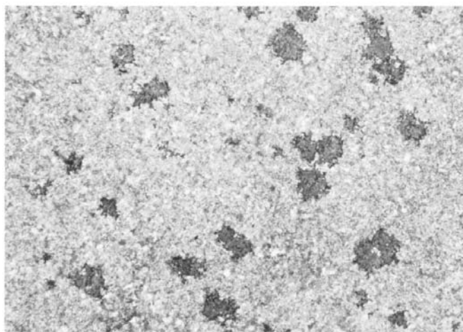
FIG. X1.6 Grade M8501 Approximately HB 285 (100×)
