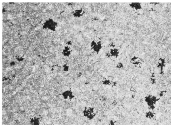
FIG. X1.5 Grade M7002, Approximately HB 262 (100x)
