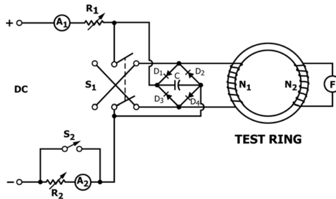
FIG. X2.1 Schematic Illustration of Arc Suppression Diode Bridge Placed in the Circuit Shown in Fig. 1
