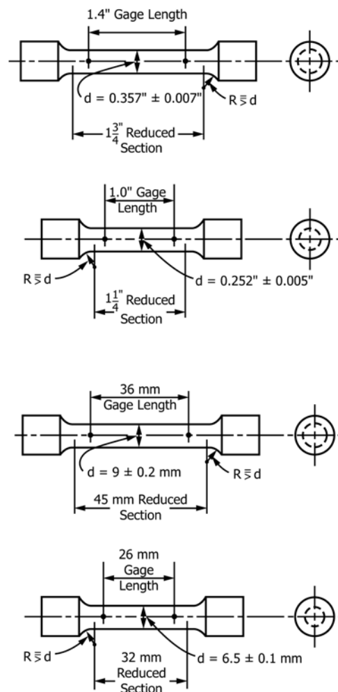
FIG. 5 Examples of Small-Size Specimens Proportional to Standard \frac{1}{2} -in. [12.5-mm] Round Specimen
