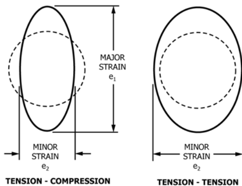
FIG. X4.2 Major and Minor Strain Axes
