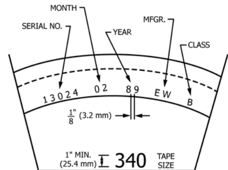
FIG. 2 Typical Reference Standards for Rim Tread Test (Radial Testing)
