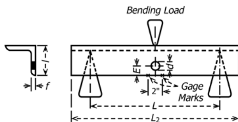
NOTE 1—2 in. = 51 mm. FIG. 1 Specimen for Elongation after Fracture
