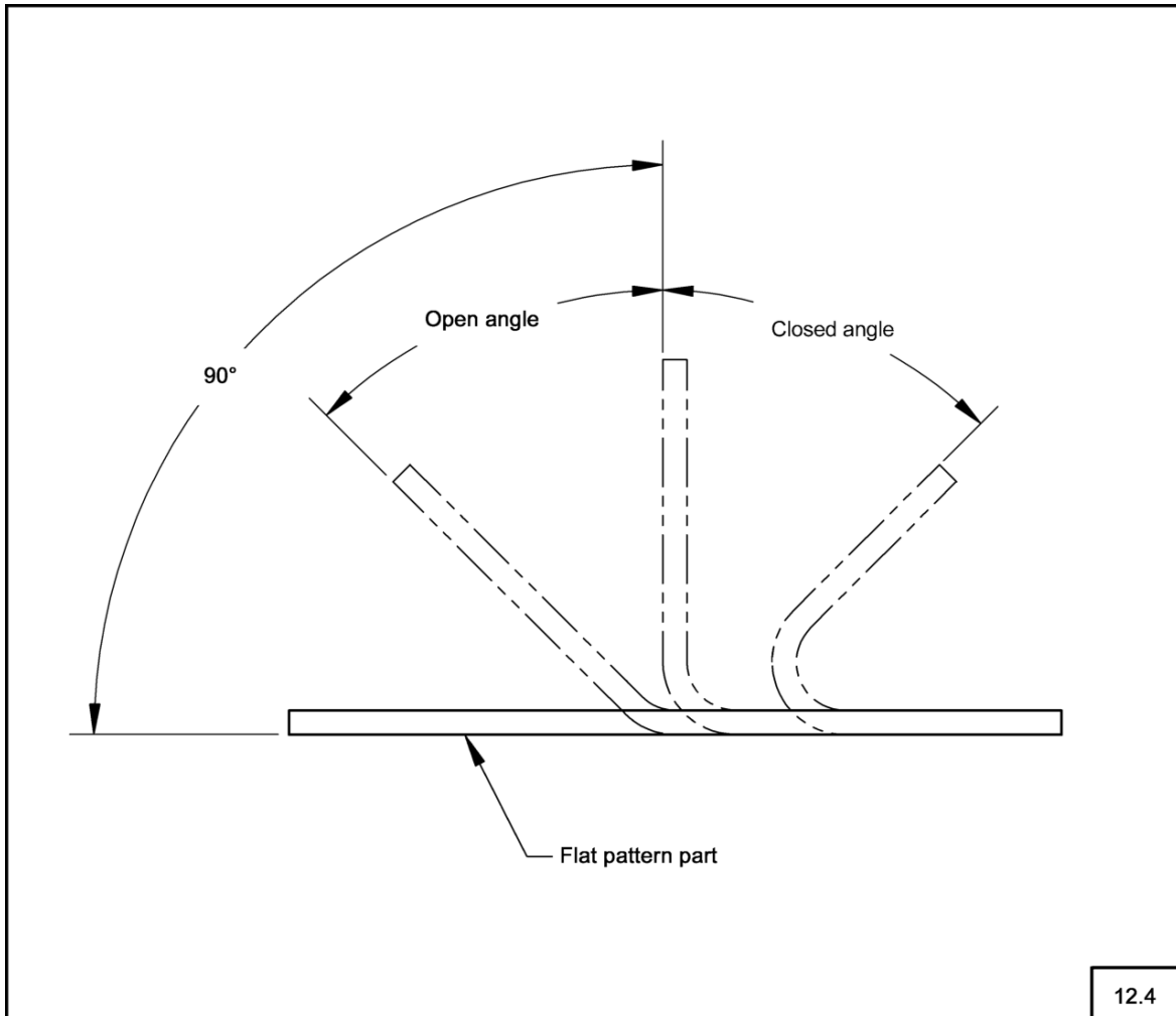
Fig. 12-3 Flange Angle Examples
