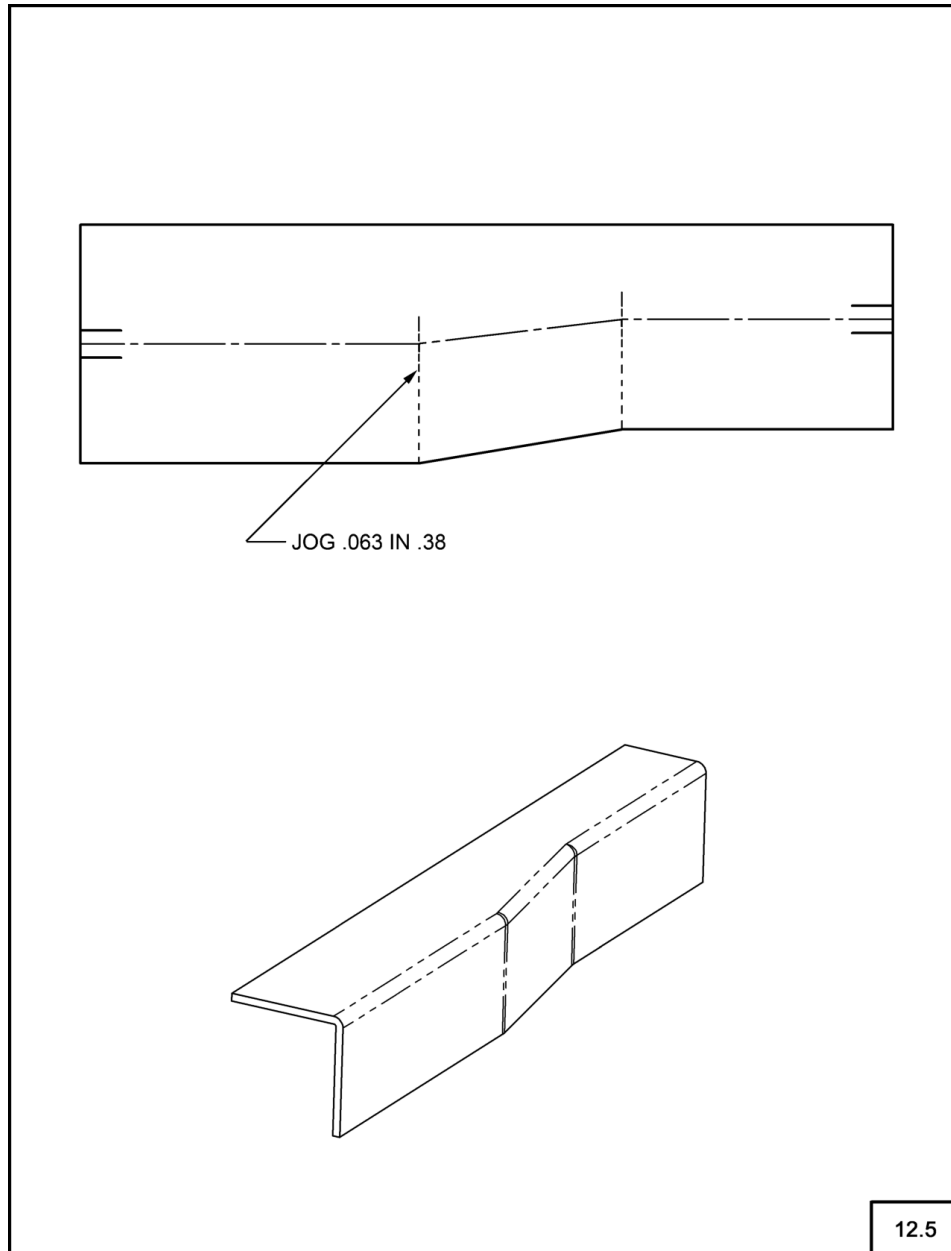
Fig. 12-7 Hydro Joggle Example
