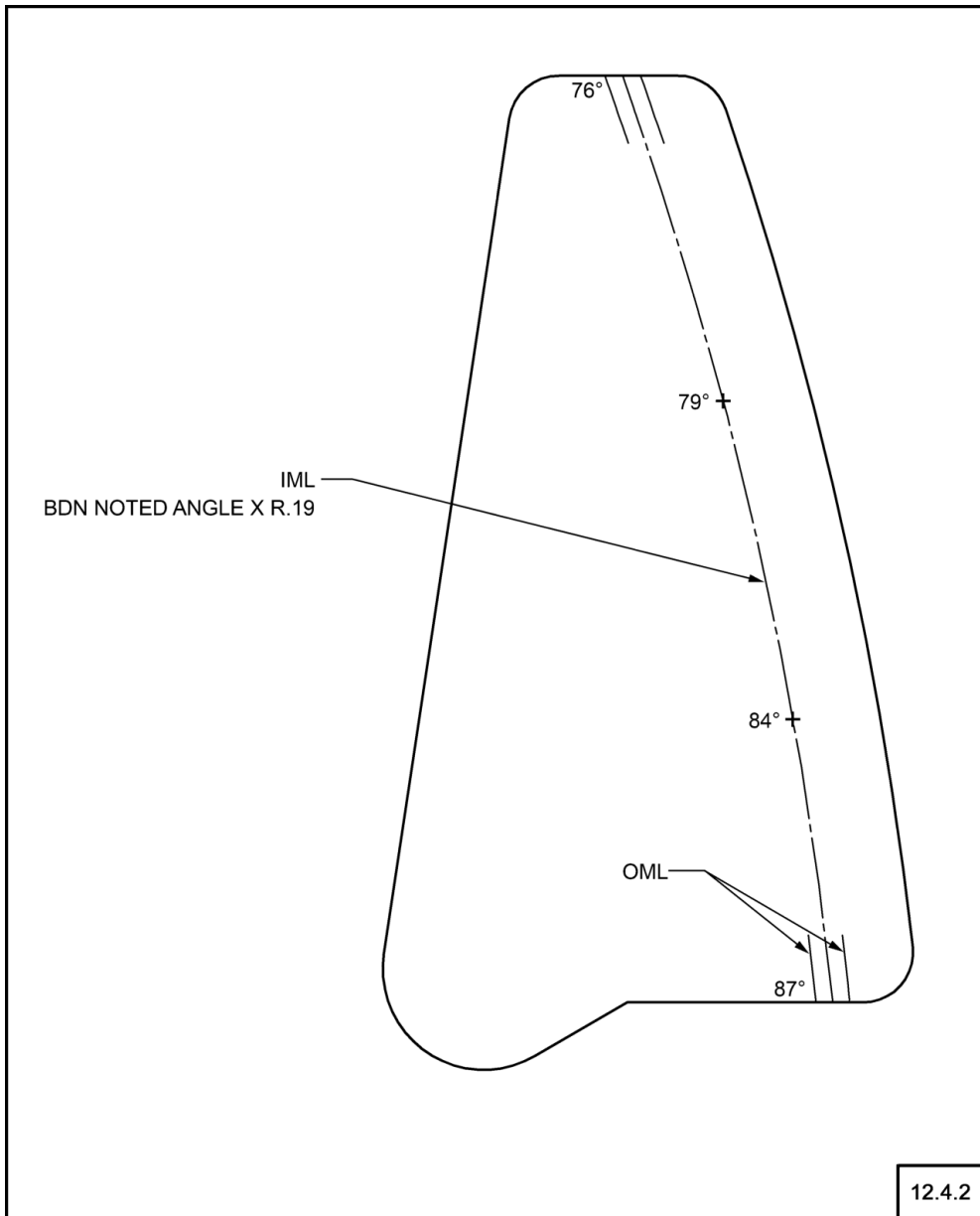
Fig. 12-4 Variable Bend Angle Example
