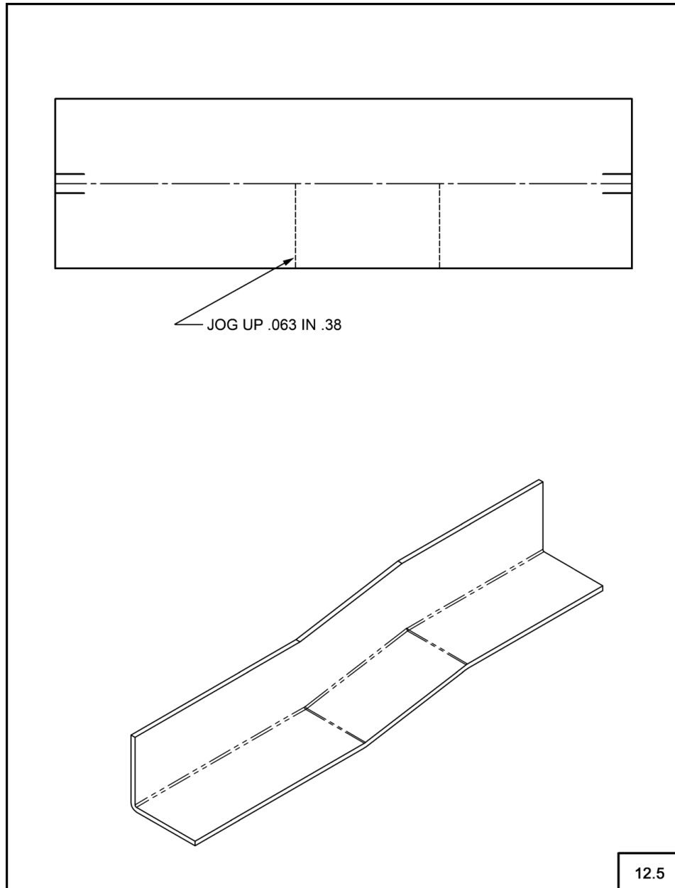
Fig. 12-5 Joggle Material Displacement Example 1
