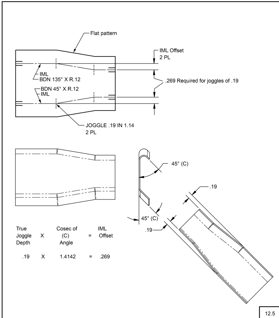
Fig. 12-8 Hydro Joggle Offset Example
