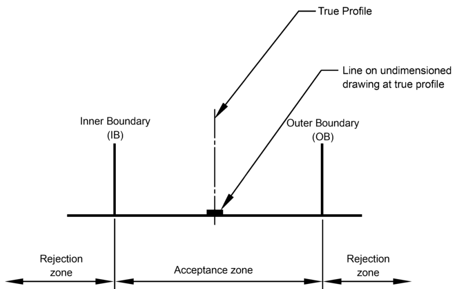
(a) Linework at true profile
