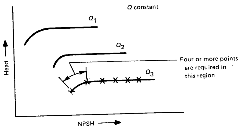
FIG. 4.43.1 CONSTANT CAPACITY
