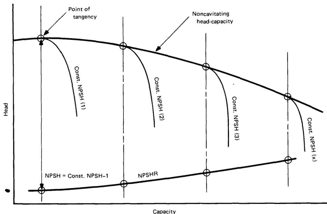
FIG. H3 NPSH TEST RESULTS FOR CONSTANT NPSH VALUES
