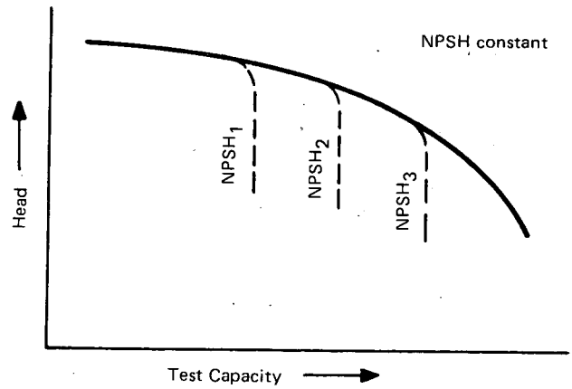
FIG. 4.44.1 CONSTANT NPSH
