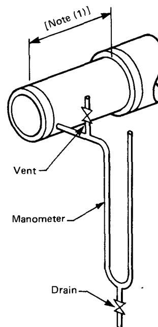
NOTE: (1) See para. 4.7 for pipe dimensions.
