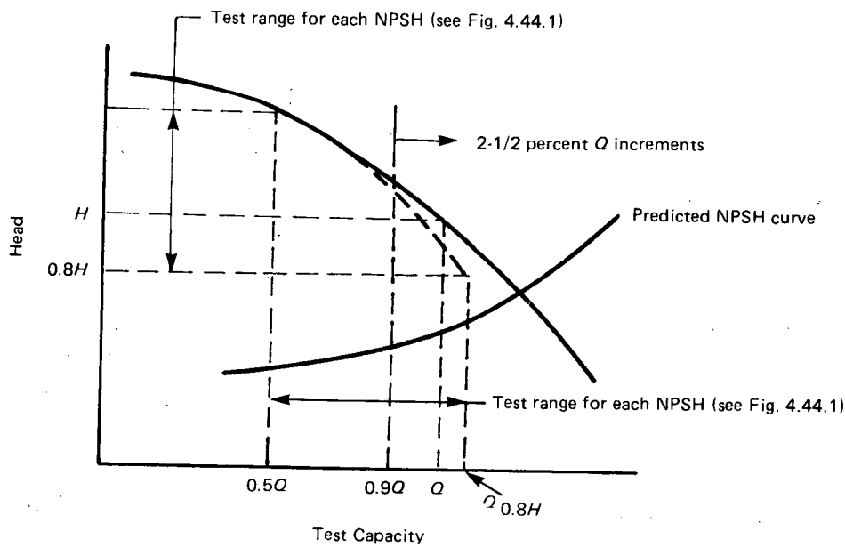
FIG. 4.44.2 CONSTANT NPSH
