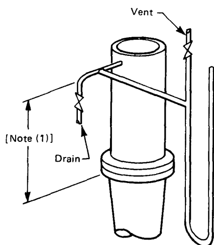
NOTE: (1) See para. 4.7 for pipe dimensions.
