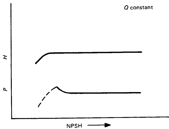
FIG. 4.43.2 CONSTANT CAPACITY
