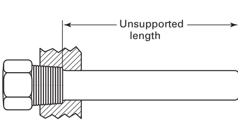
(a) Threaded Thermowell
