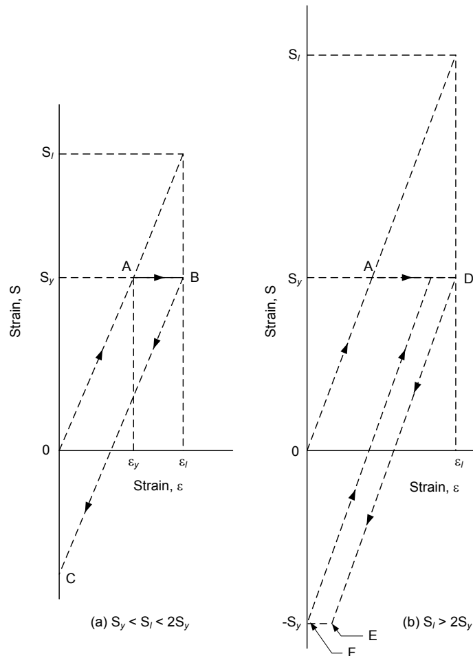
Figure 3 – Strain History Beyond Yield
