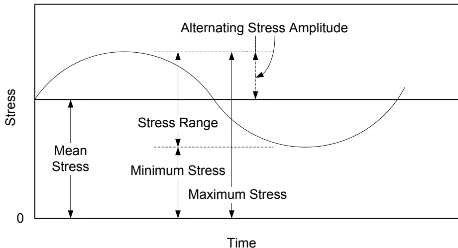
Figure 5 – Stress Fluctuation Around a Mean Value
