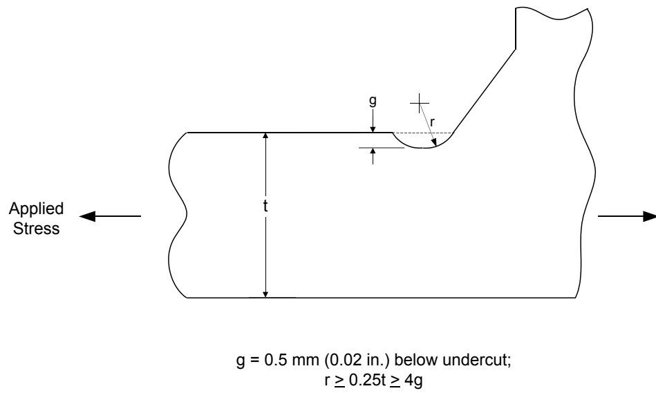
Figure 5-28: Weld Toe Dressing by Burr Grinding
