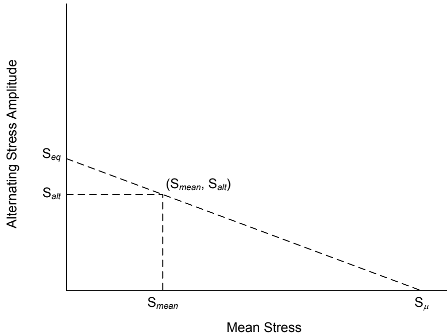
Figure 7 – Graphical Determination of S_{eq}
