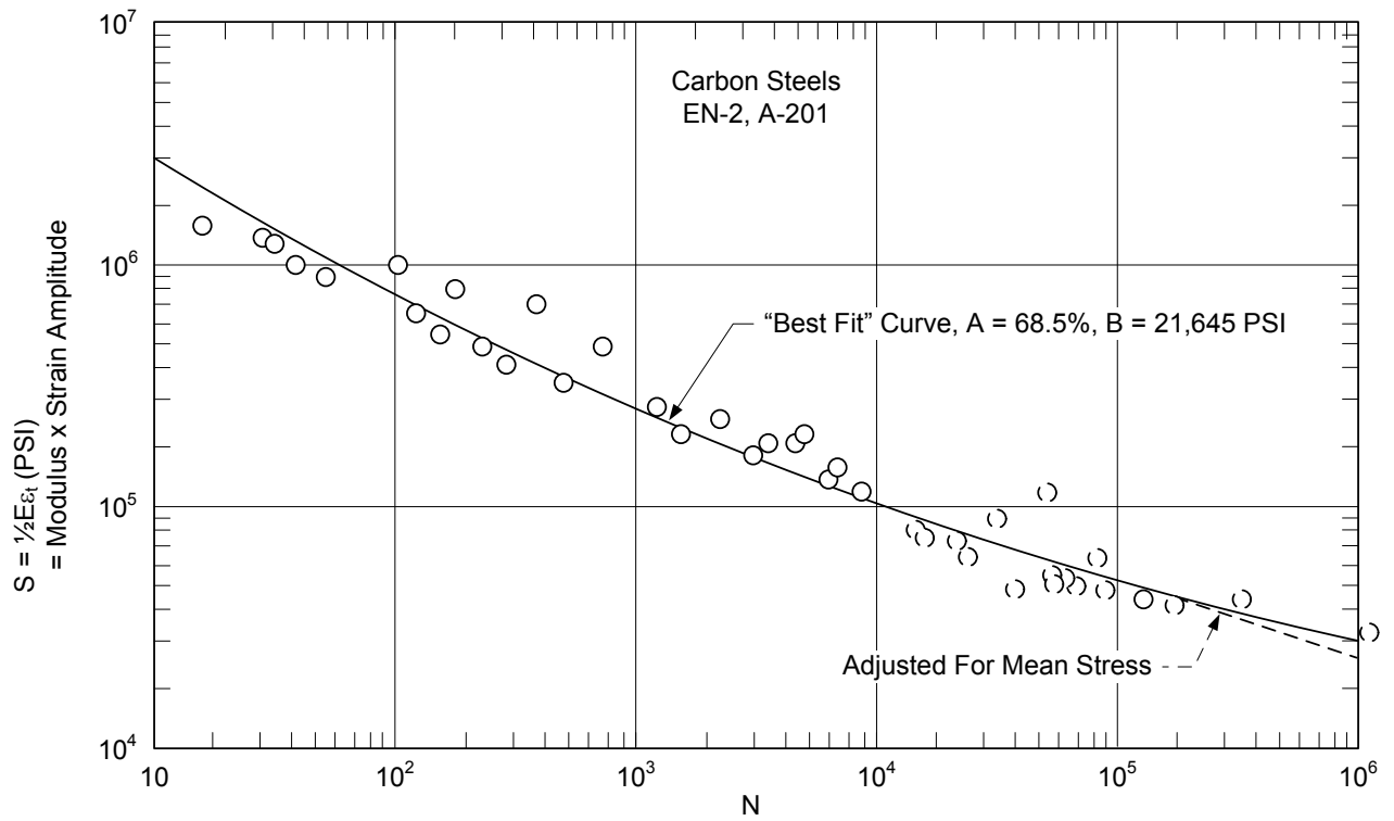
Figure 9 – Fatigue Data - Carbon Steels
