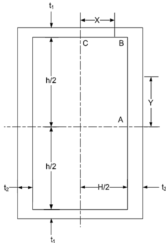
Figure 4-29: (VIII-2 Figure 4.12.1) – Type 1 Noncircular Vessels (Rectangular Cross Section)
