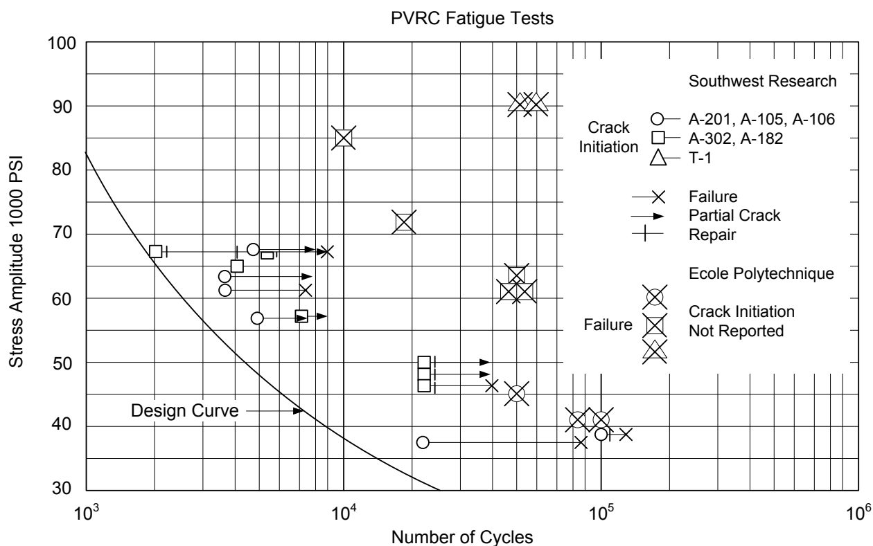
Figure 12. - PVRC Fatigue Tests
