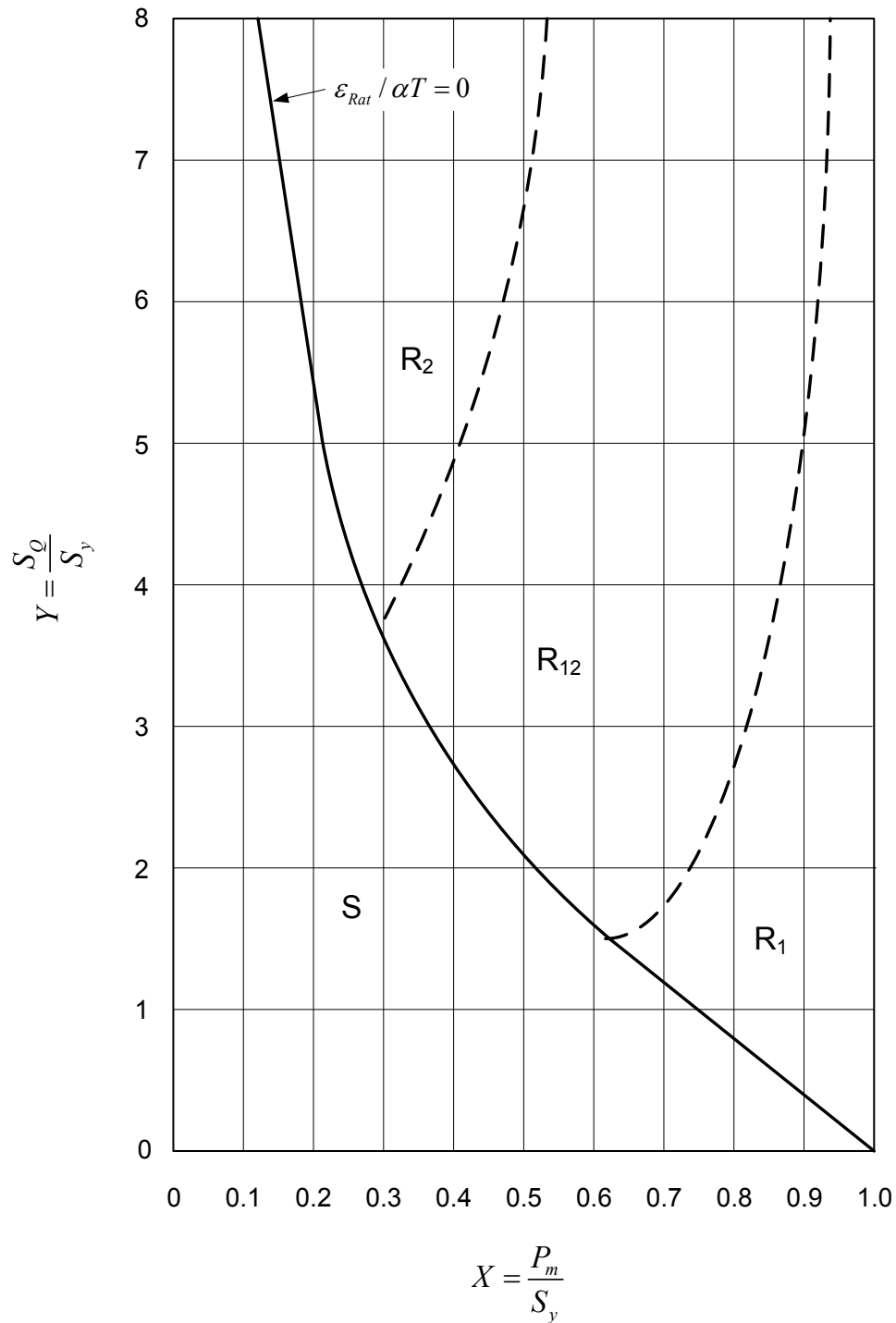
Figure 5-31: Allowable Secondary Equivalent Stress Range from Thermal Loading with a Parabolic Constantly Increasing or Decreasing Variation Through the Wall Thickness
