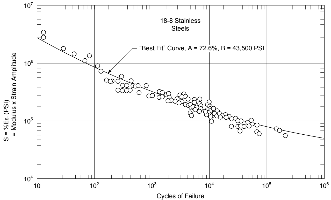
Figure 11 – Fatigue Data - Stainless Steels
