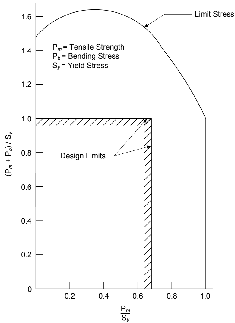
Figure 2 – Limit Stress for Combined Tension and Bending (Rectangular Section)
