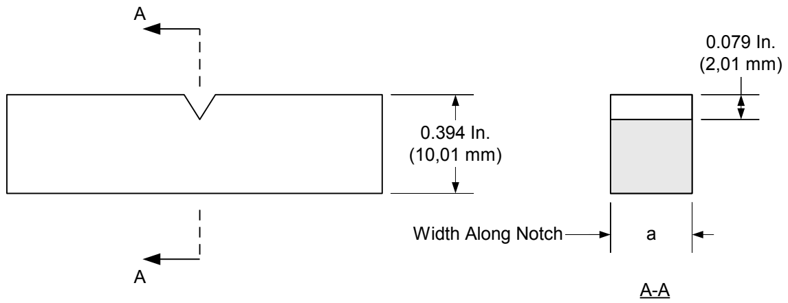
Figure 3-14: (VIII-2 Figure 3.5) – Illustration of Lateral Expansion in a Broken Charpy V-Notch Specimen
