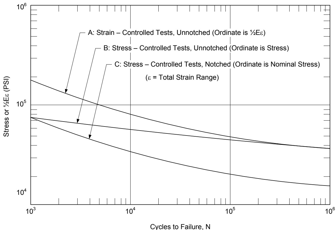
Figure 4 – Typical Relationship Between Stress, Strain, and Cycles-to-Failure
