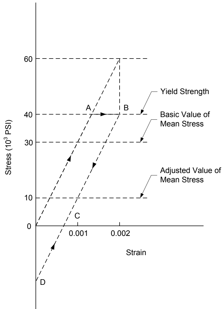
Figure 8 – Idealized Stress versus Strain History
