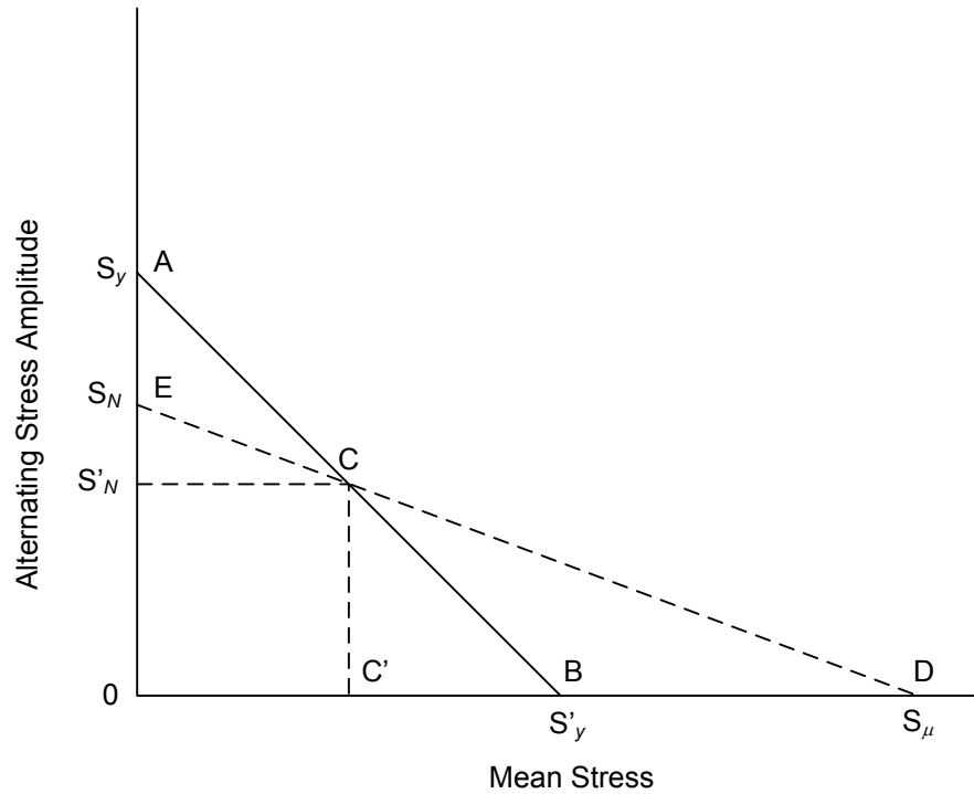
Figure 6 – Modified Goodman Diagram
