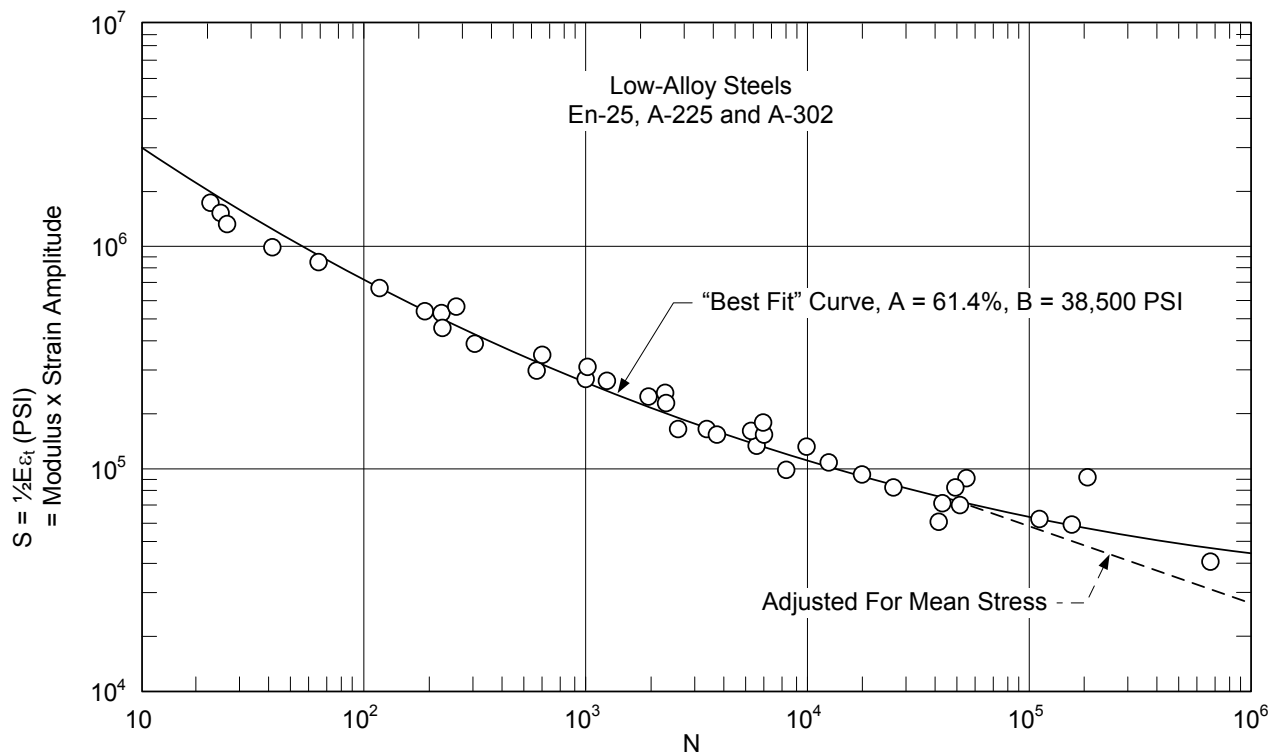
Figure 10 – Fatigue Data - Low Alloy Steels
