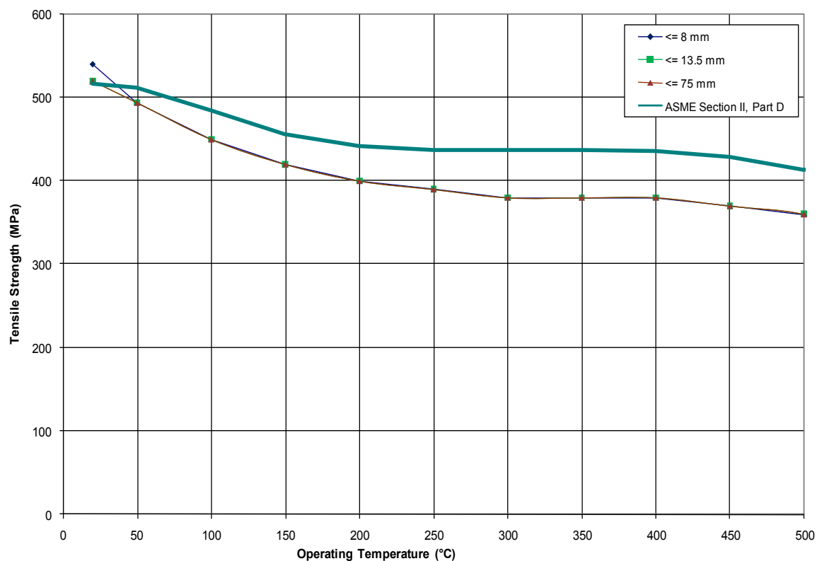
Figure 3-27: SA 240 Type 304 and X5CrNi18-10 – Tensile Strength
