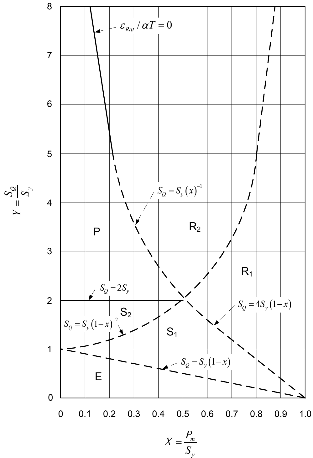
Figure 5-30: Allowable Secondary Equivalent Stress Range from Thermal Loading with a Linear Variation Through the Wall Thickness
