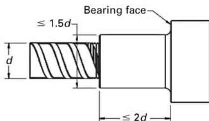
(15) Figure CC-2310-1 Maximum Dimensions of Obstruction or Interruptions of Bar Deformations and Nonplanar Features of the Bearing Face
