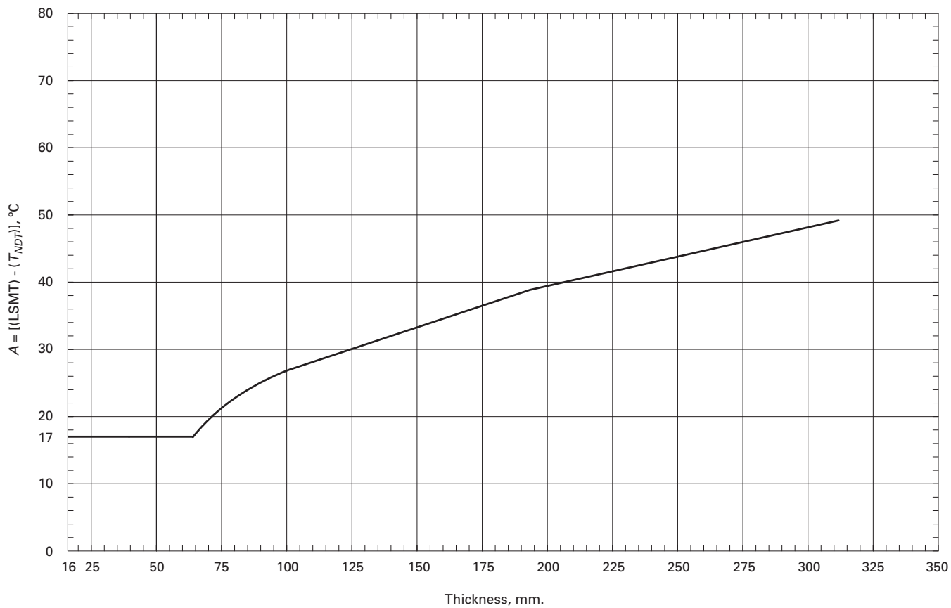
Figure CC-2521.1-1M Determination of Permissible Lowest Service Metal Temperature
