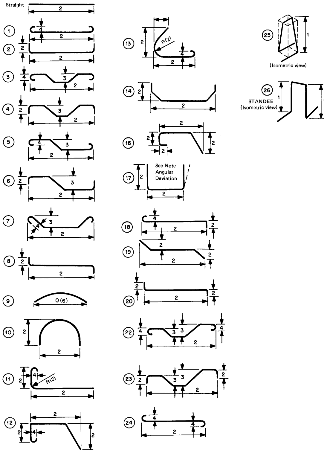
Figure D2-F-1220-1 Standard Fabricating Tolerances for Bar Sizes #3 (10 mm) Through #11 (35 mm)
