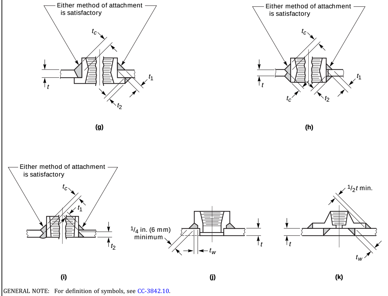
Figure CC-4542.2-2 Typical Category D Joints for Nozzle Diameters NPS 3 (DN 80) and Less (Cont'd)
