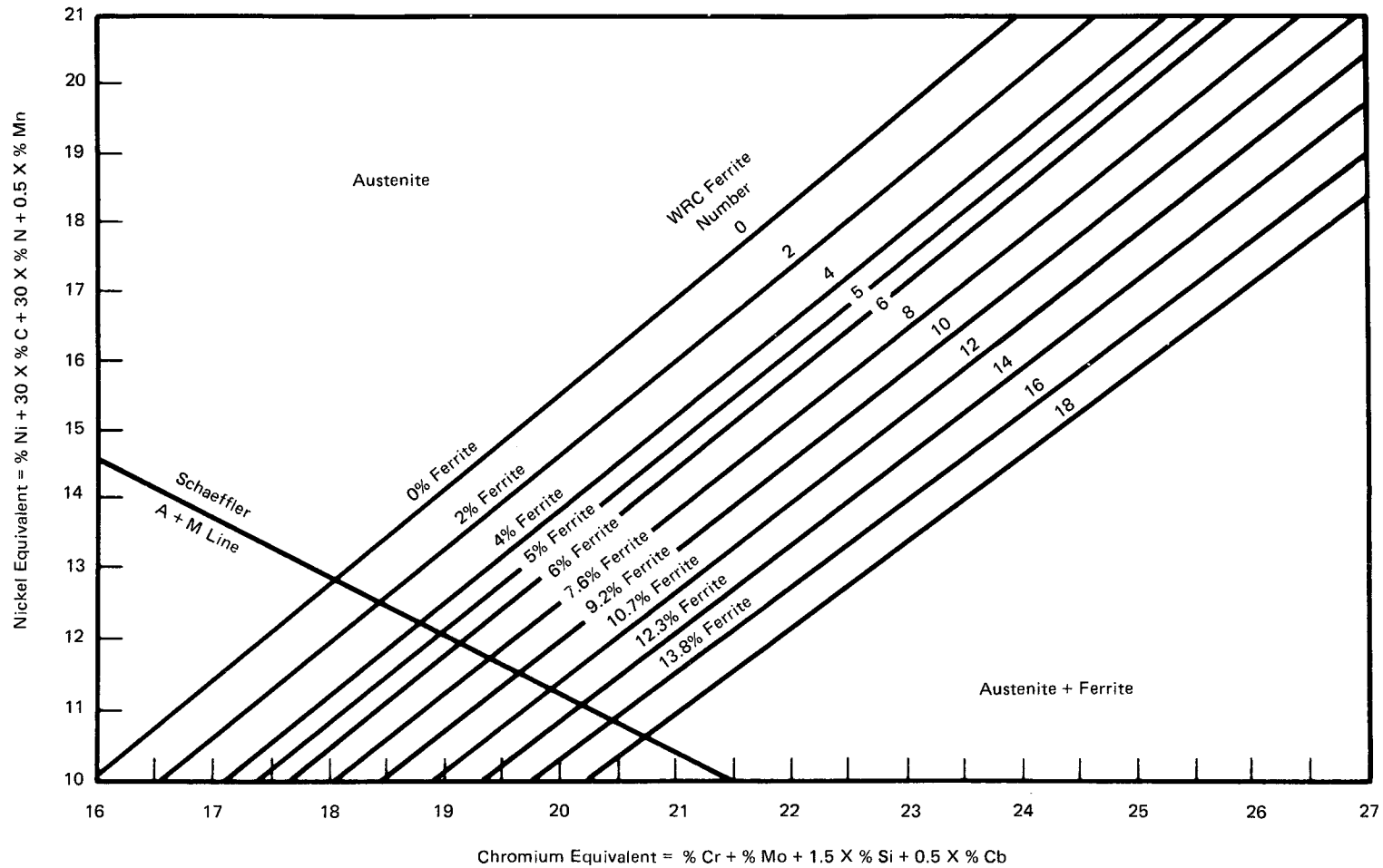
Figure CC-2613.3.1-1 Delta Ferrite Content
