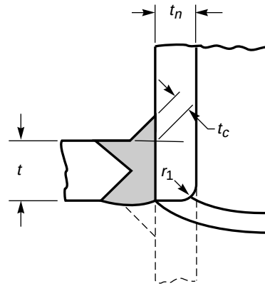
Figure CC-4542.2-1 Typical Category D Joints for Nozzle Diameters Over NPS 3 (DN 80) (Cont'd)
