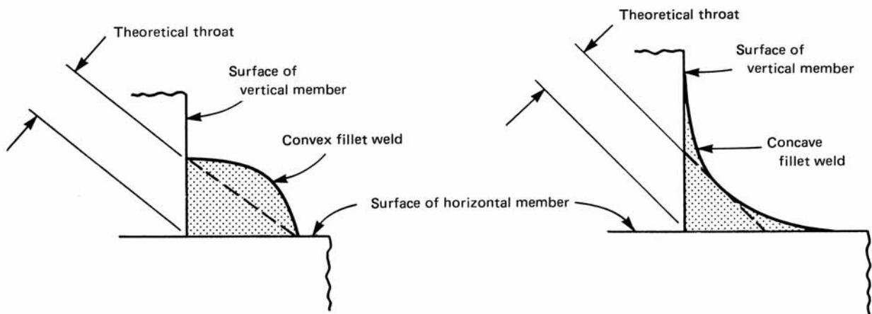
Unequal Leg Fillet Weld [Note (2)]
