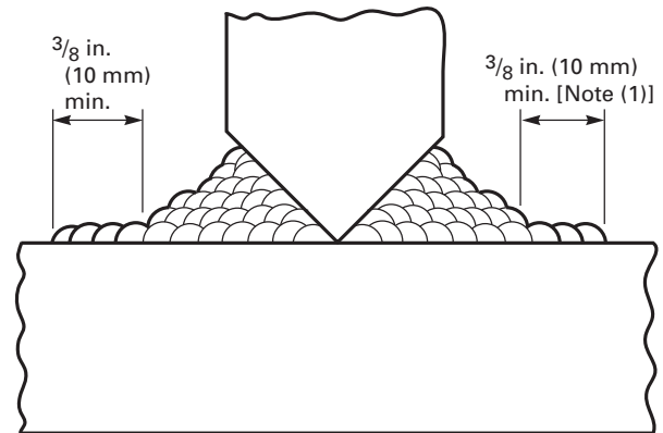
Figure CC-4543.6-2 Special Deposition Technique for Weld Joint Producing Through-Thickness Loading (Typical)
