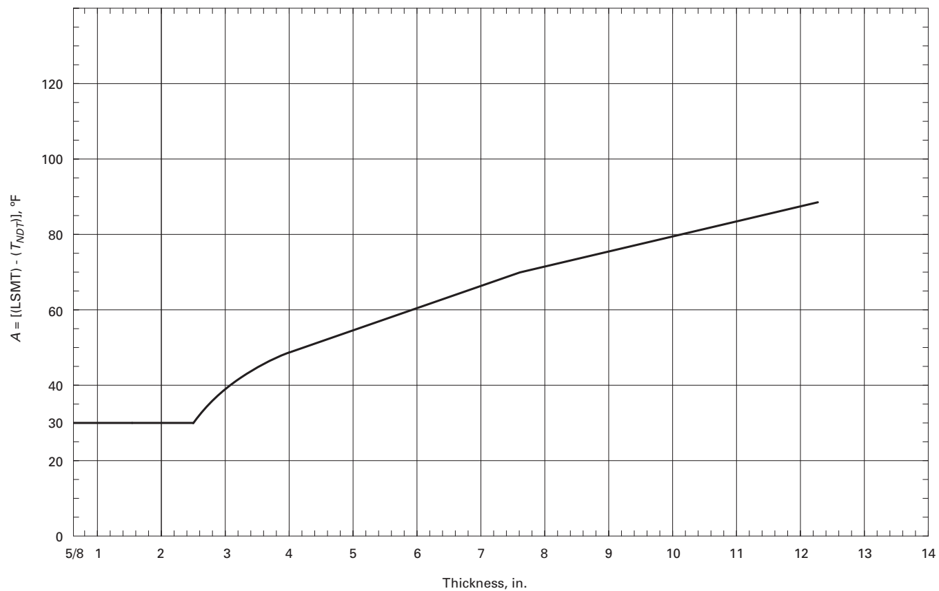
Figure CC-2521.1-1 Determination of Permissible Lowest Service Metal Temperature
