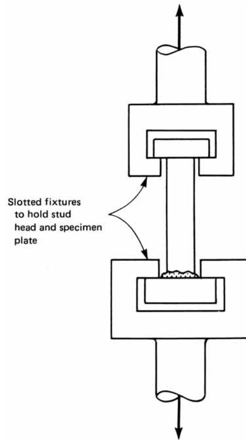
Figure CC-2620-2 Typical Tensile Test Fixture
