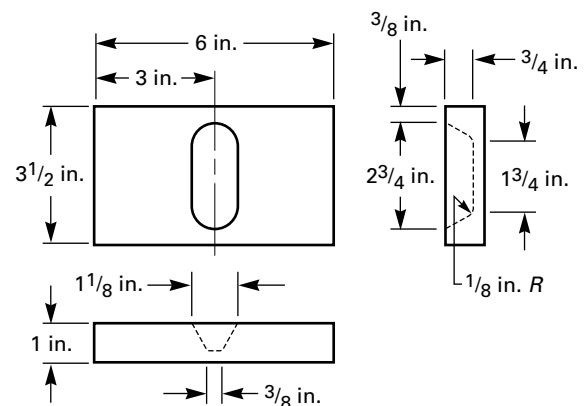
FIG. 1 CAST BLOCK FOR WELDABILITY TEST
