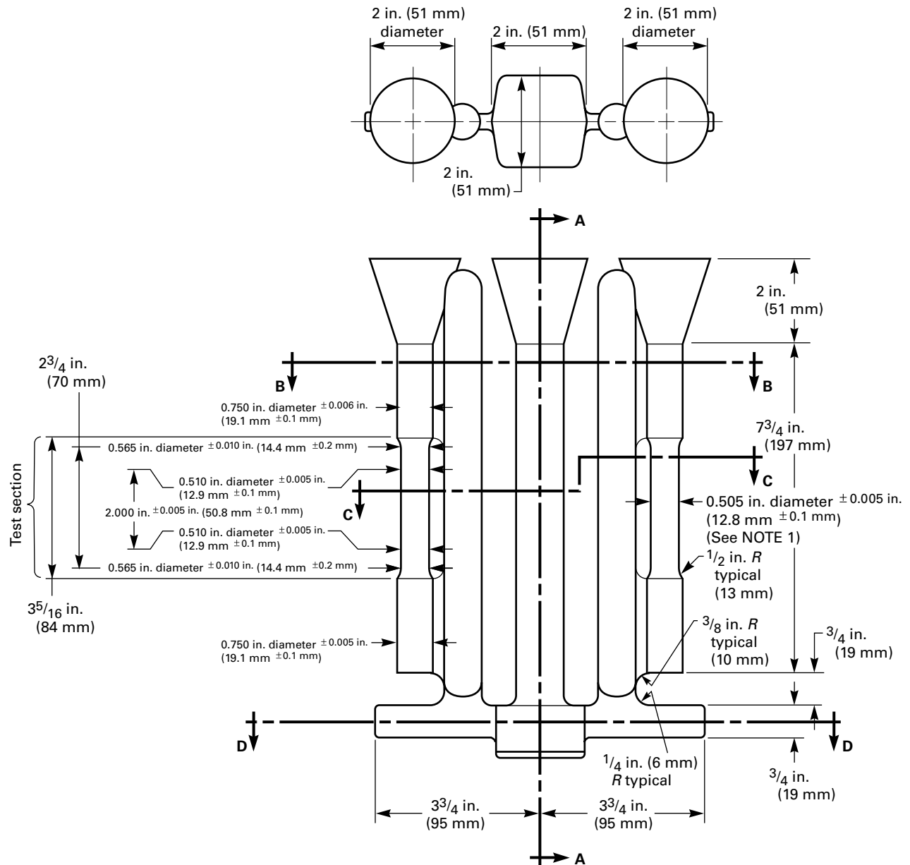
FIG. 1 TENSION TEST SPECIMEN CASTING
