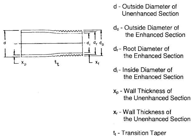
FIG. 1 Outside Diameter Enhanced Tube Nomenclature
