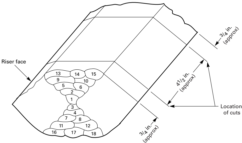
FIG. 3 X-WELD TEST
