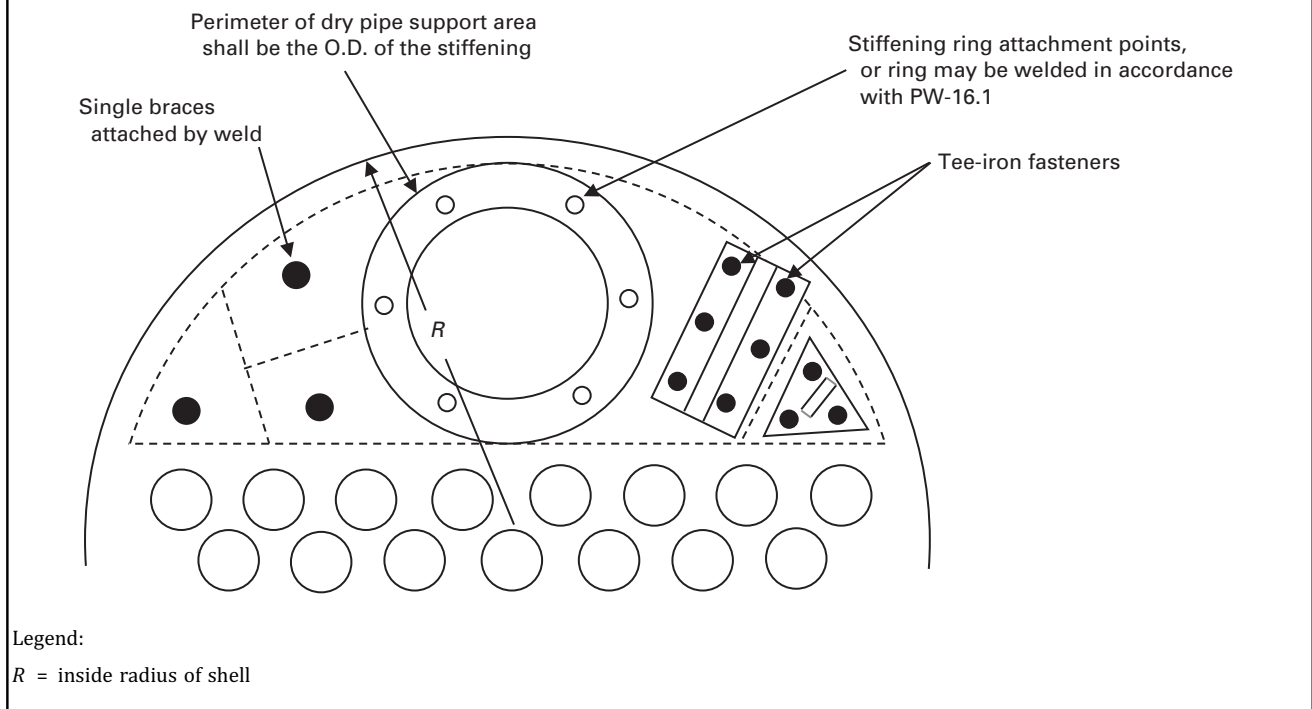
Figure PL-36.2.1-1 Support Perimeters
