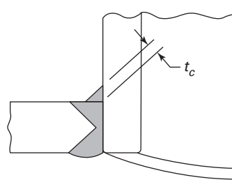
(h) Typical Flush-Type Nozzle
