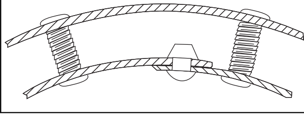
Figure V-2.2-2 Proper Location of Staybolts Adjacent to Longitudinal Joint in Furnace Sheet
