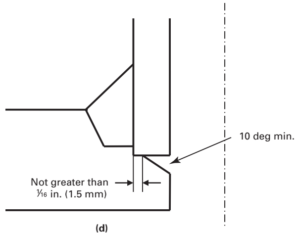
Figure PW-16.8 Some Acceptable Designs for Partial-Penetration-Weld-Type Attachments Designed for 900°F (480°C) or Higher Service (Cont'd)
