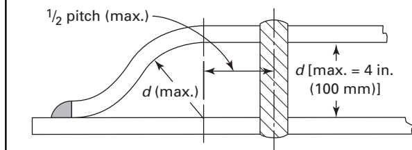
Figure PFT-20 Welding Ogee Ring
