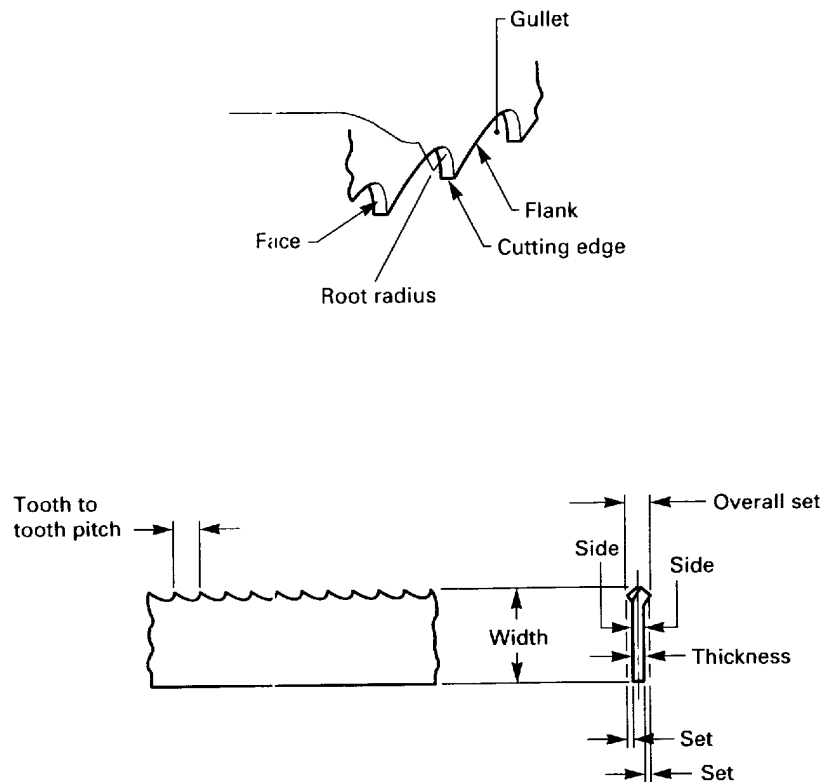
FIG. 2 TOOTH FEATURES
