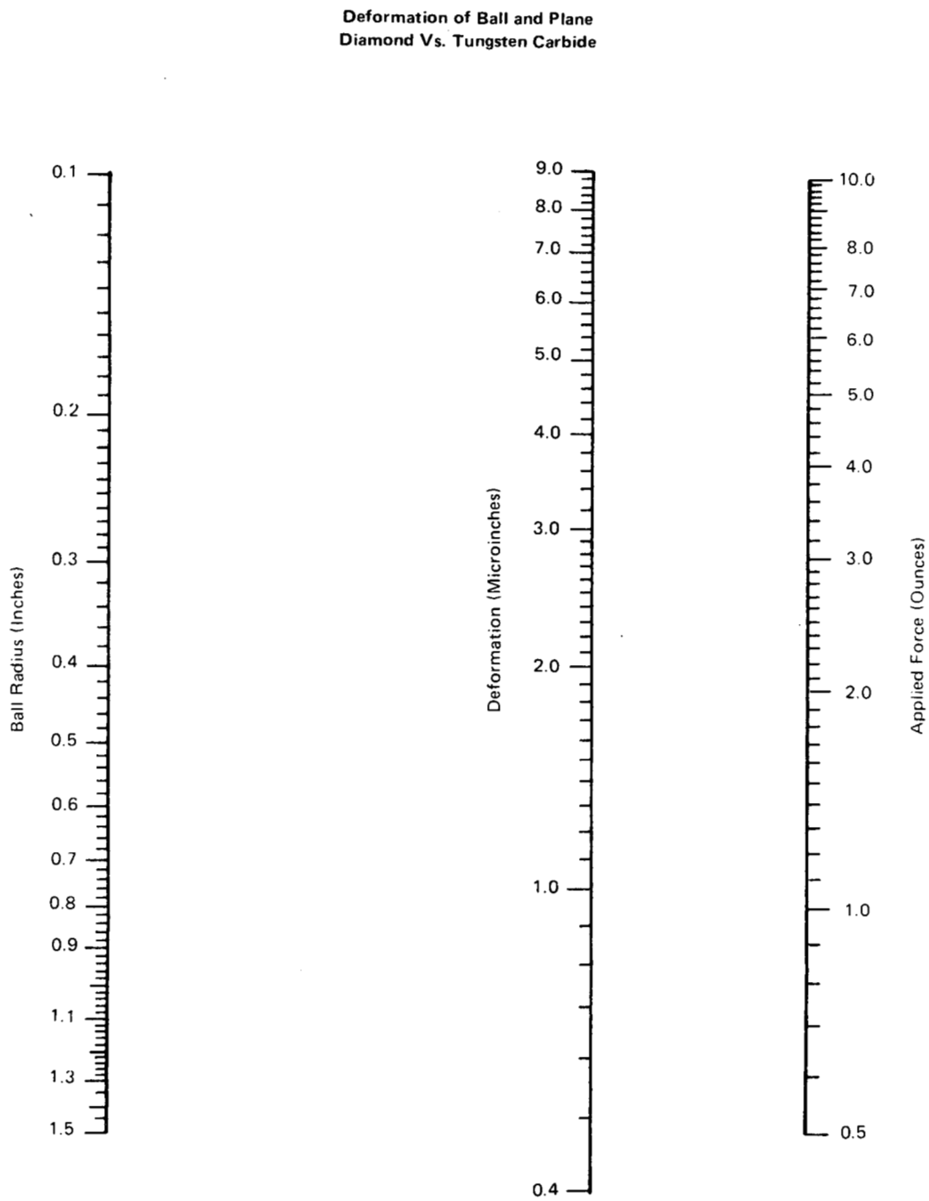
FIG. B1.1 DEFORMATION OF BALL AND PLANE — DIAMOND VS. TUNGSTEN CARBIDE
