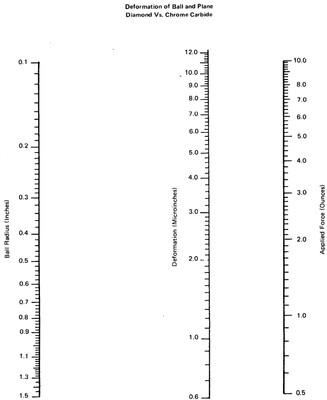
FIG. B1.2 DEFORMATION OF BALL AND PLANE — DIAMOND VS. CHROME CARBIDE
