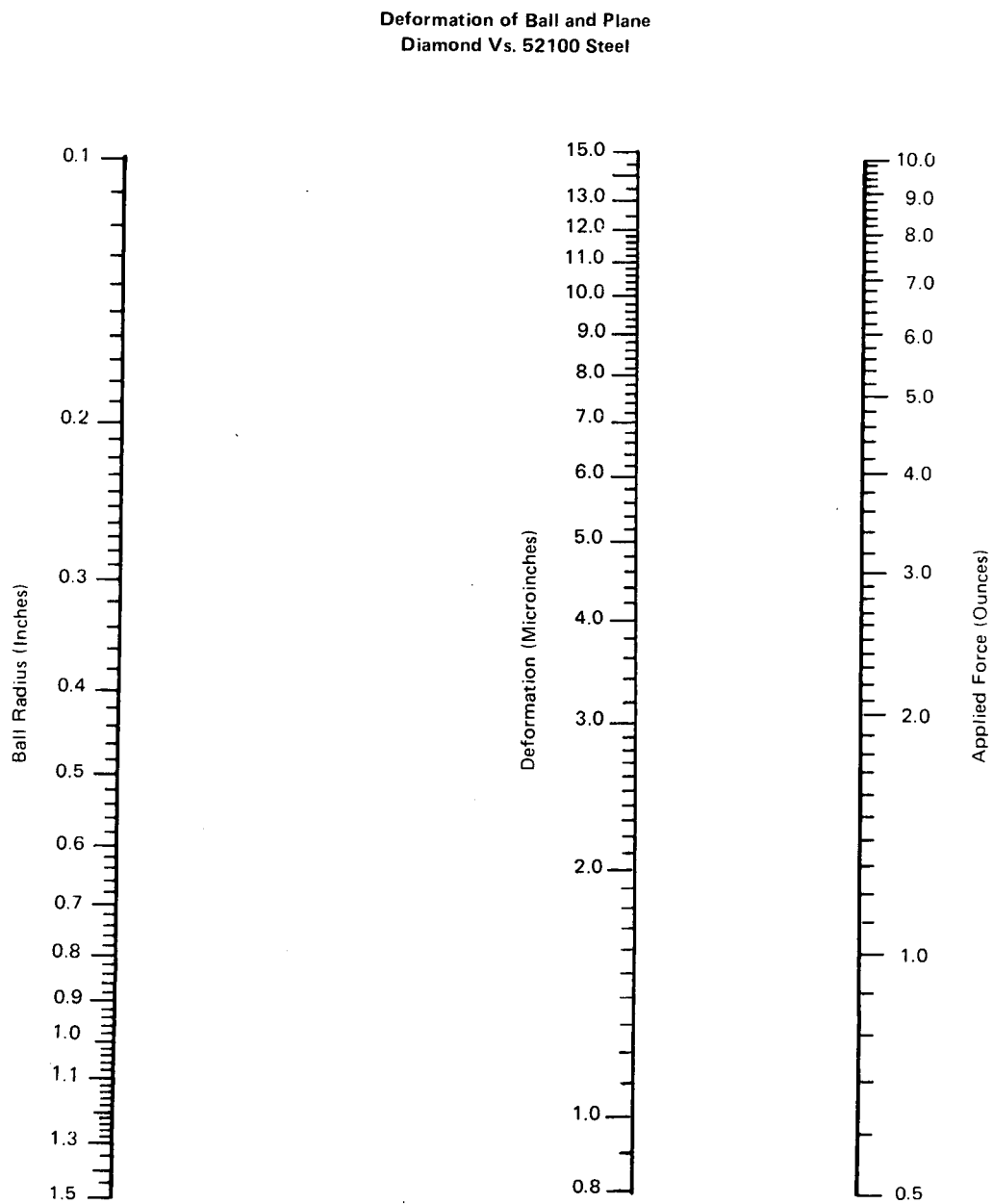
FIG. B1.3 DEFORMATION OF BALL AND PLANE — DIAMOND VS. 52100 STEEL
