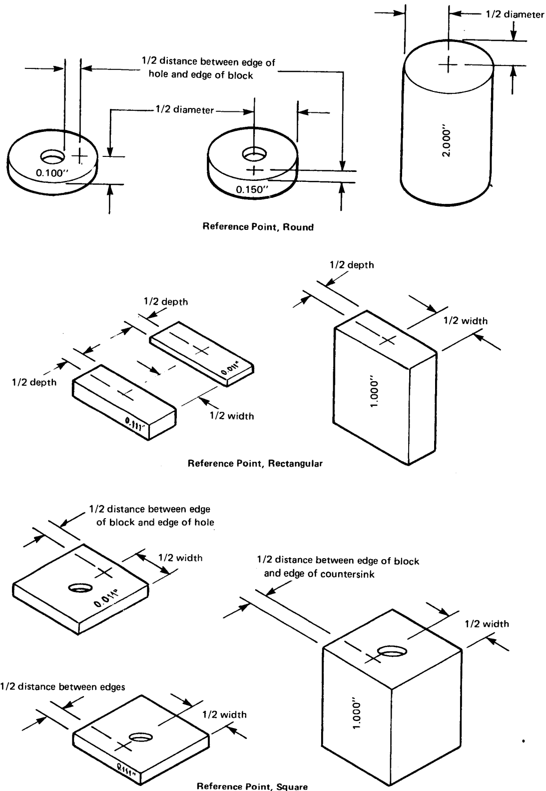
FIG. 1 GAGE BLOCK REFERENCE POINTS
