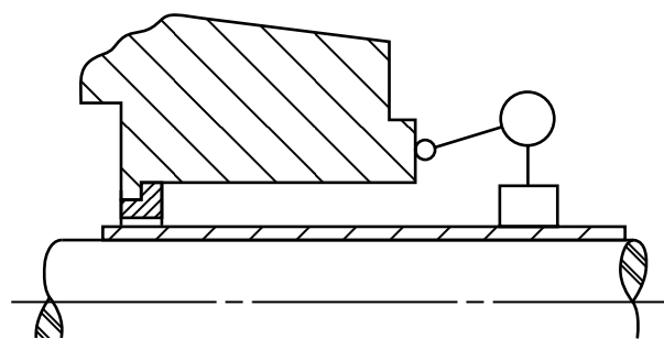
FIG. 8 SEAL CHAMBER FACE RUNOUT
