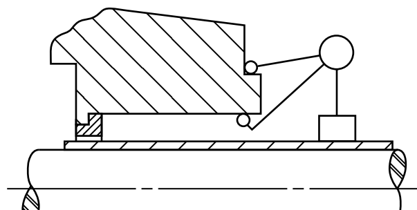
FIG. 9 SEAL CHAMBER REGISTER CONCENTRICITY
