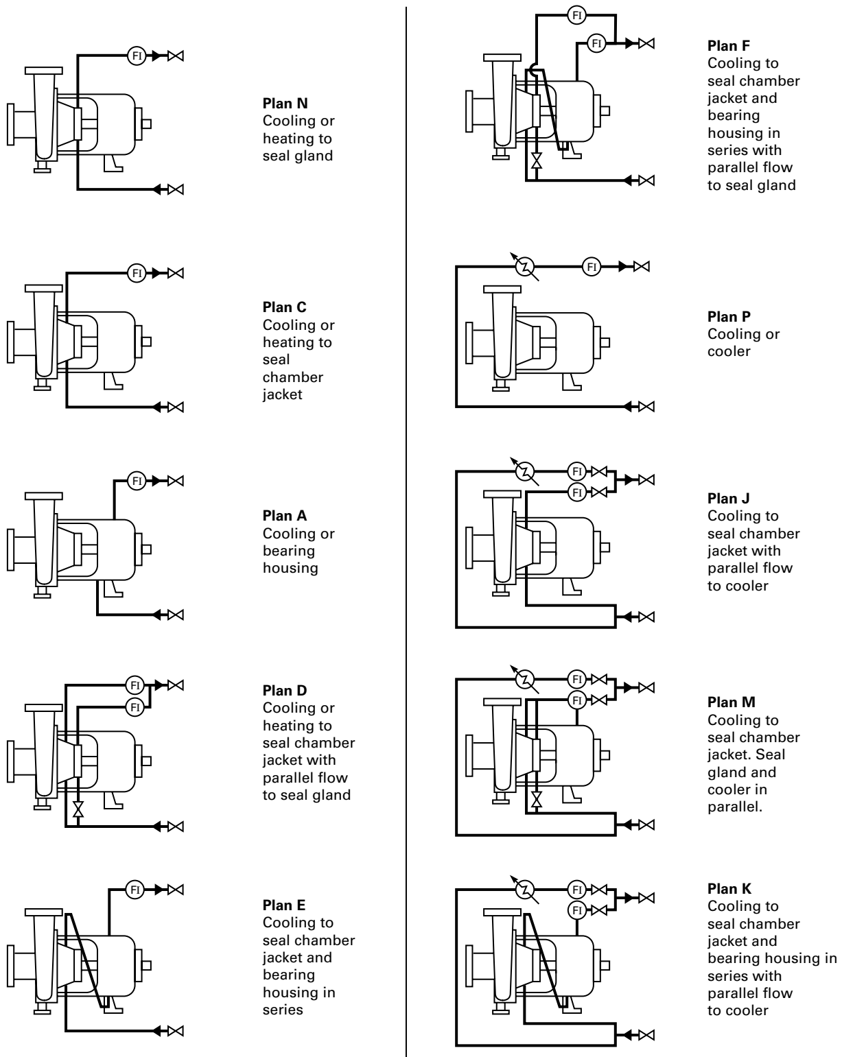
FIG. 3 COOLING AND HEATING PIPING PLANS
