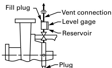
Plan No. 7351 Dead-ended blanket
