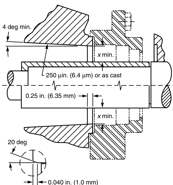
Lead chamfer for o-ring and other sealing devices
