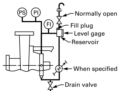
Plan No. 7352 External fluid reservoir for tandem seals. thermosyphon or forced circulation, as required. [Note (1)]
