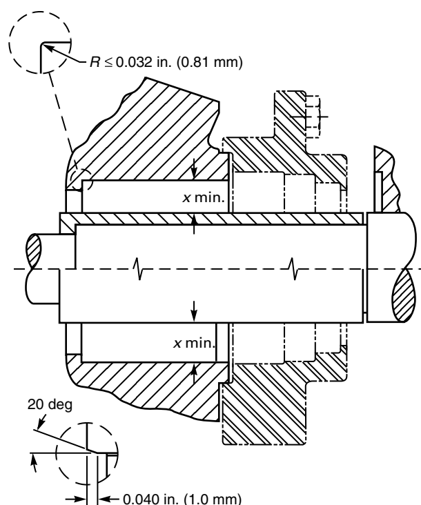
Lead chamfer for o-ring and other sealing devices
