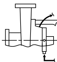
Plan No. 7354 Circulation of clean buffer fluid from an external source. [Note (1)]
