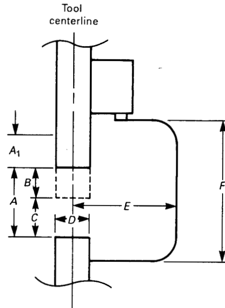
FIG. 2 PRESS BRAKE WORK AREA DIMENSIONS
