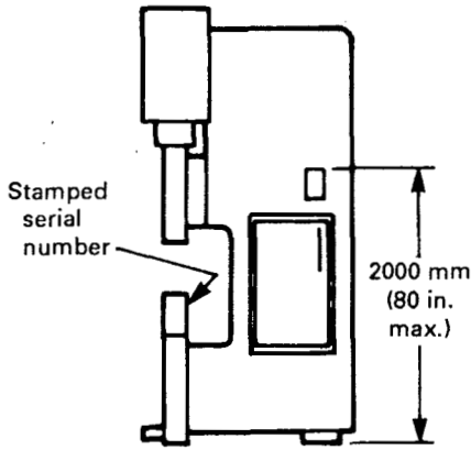
FIG. 11 NAMEPLATE LOCATION
