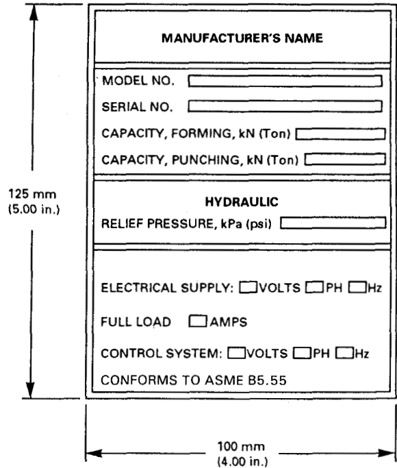
FIG. 12 DATA PLATE
