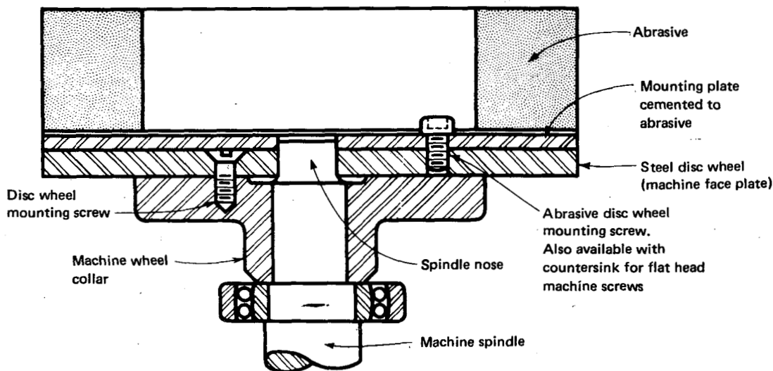
FIG. 6 TYPICAL PLATE TYPE MOUNTING
