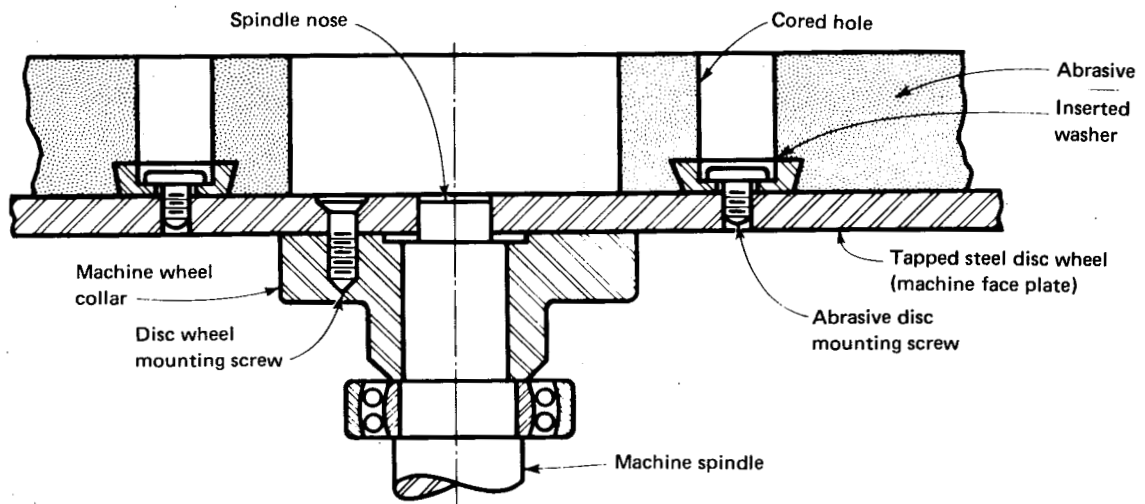
FIG. 2 TYPICAL INSERTED WASHER TYPE MOUNTING
