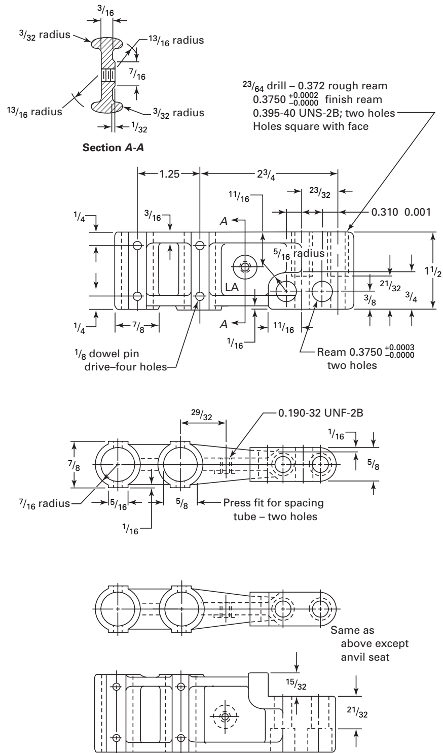
Fig. 18 Adjustable Length Gauge, Progressive, Model LB, Details of Gauge Heads
