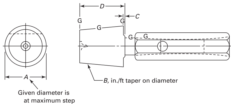
Fig. 23 Recommended Design of Taper Plug Gage for Special Applications and Method of Dimensioning
