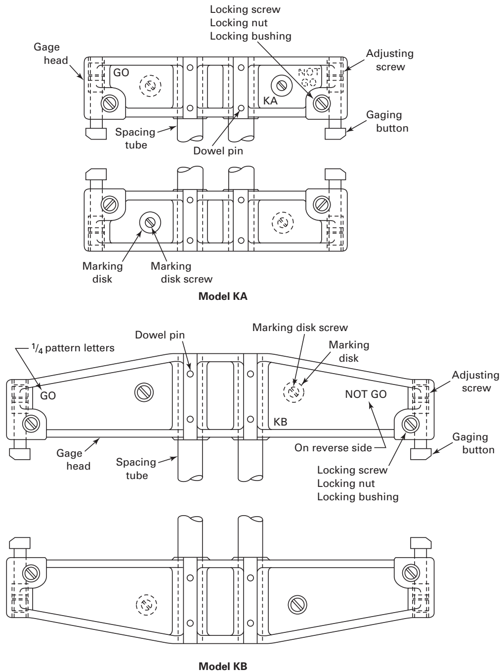
Fig. 13 Adjustable Length Gauge, Double Sided, Models KA and KB, Details of Construction
