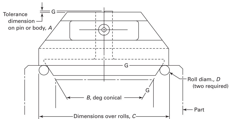
Fig. 28 Application of Countersink Type
