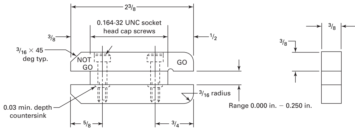
Fig. 29 Recommended Design of Small Built-Up Snap Gage
