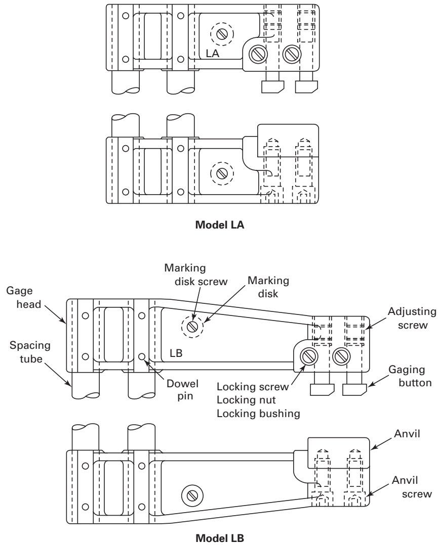
Fig. 14 Adjustable Length Gauge, Progressive, Models LA and LB, Details of Construction
