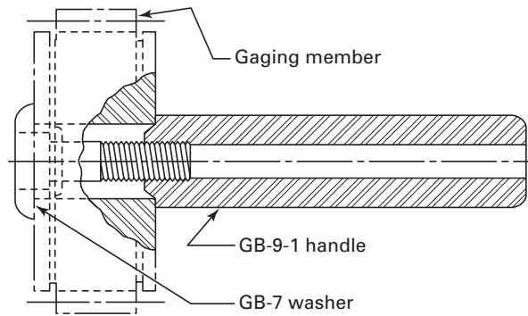
(a) Range – Above 1.5 in. to and Including 5.0 in.
