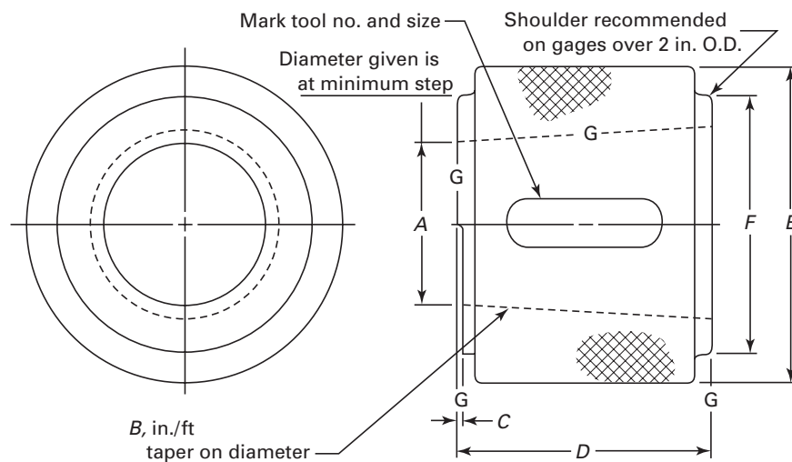
Fig. 24 Recommended Design of Taper Ring Gage for Special Applications and Method of Dimensioning
