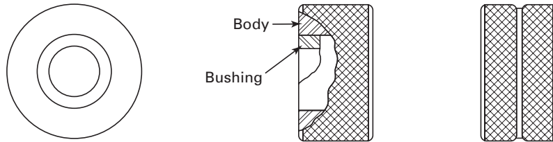
(a) Range – Above 0.010 in. to and Including 0.510 in. (Solid Design Shown Below is Optional)
