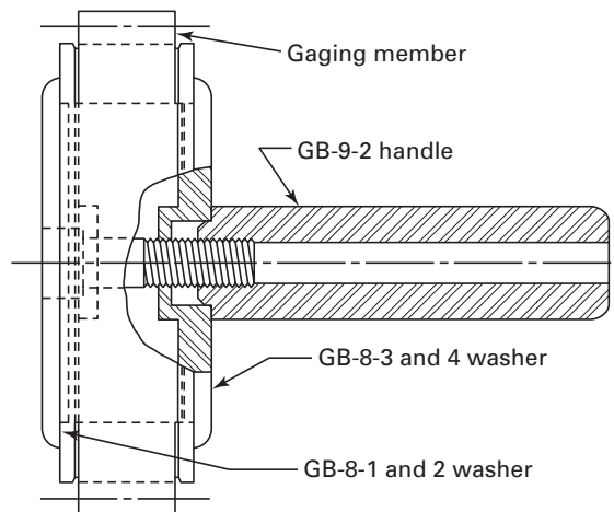
(b) Range – Above 5.0 in. to and Including 8.0 in.
