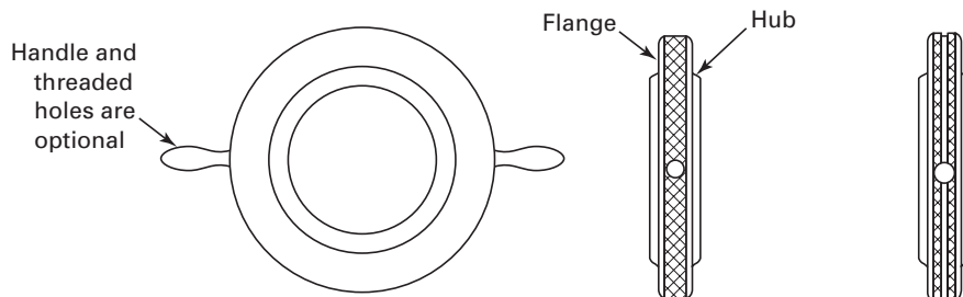
(d) Range – Above 5.510 in. to and Including 12.260 in.
