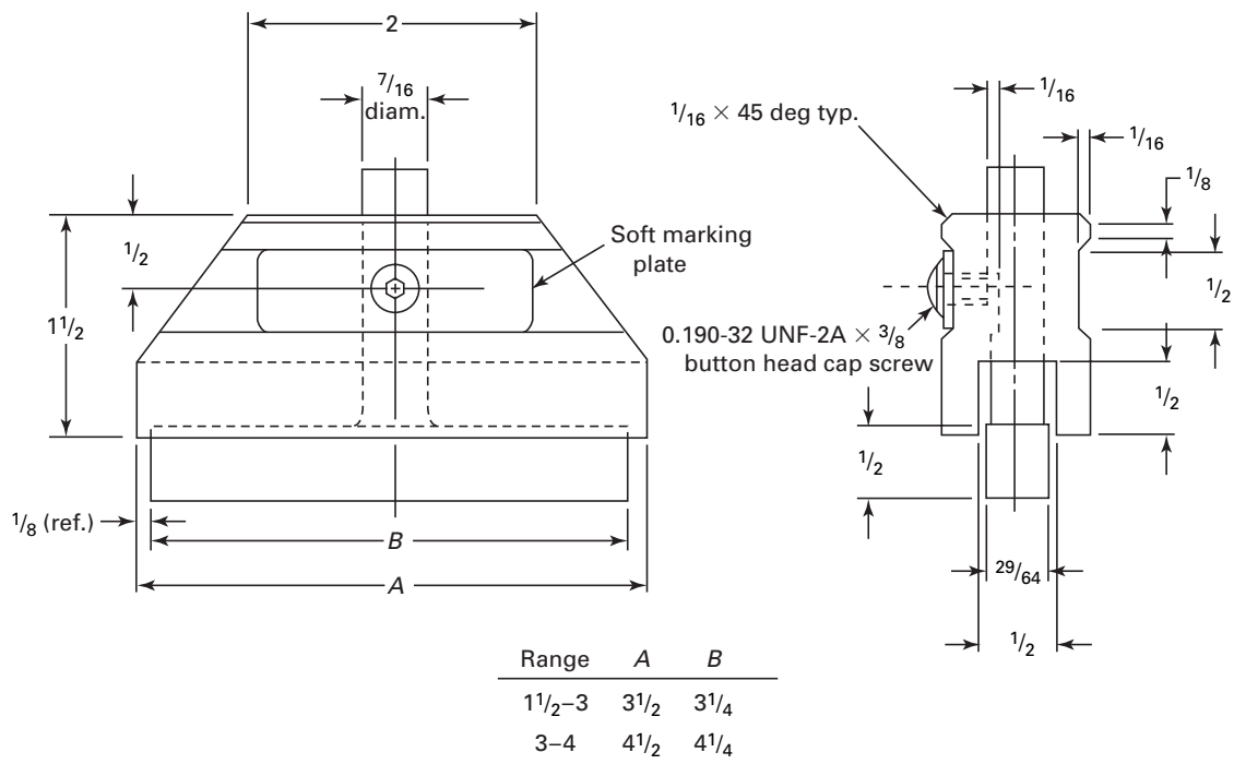
Fig. 27 Recommended Design of Large Countersink Type Flush Pin Gage
