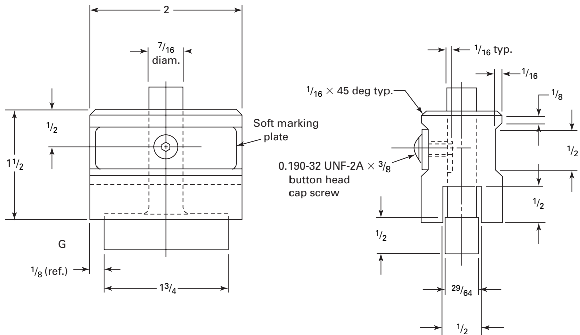
Fig. 26 Recommended Design of Small Countersink Type Flush Pin Gage — Range 3/4 in. to 1\frac{1}{2} in.
