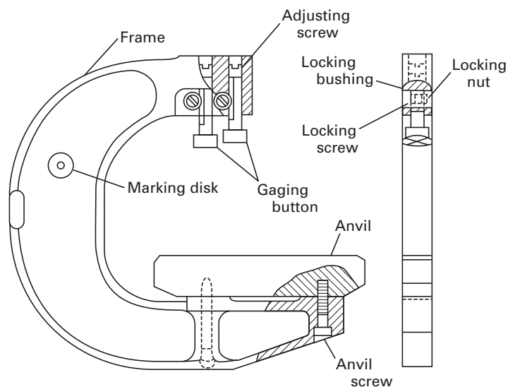
Model E: Range 0 in. to 5\frac{11}{16} in., Incl.
