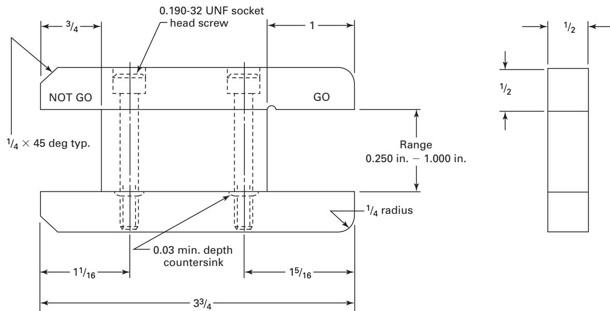
Fig. 30 Recommended Design of Large Built-Up Snap Gage
