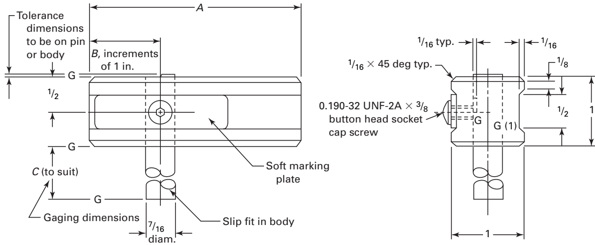
Fig. 25 Recommended Design of Bar Type Flush Pin Gage
