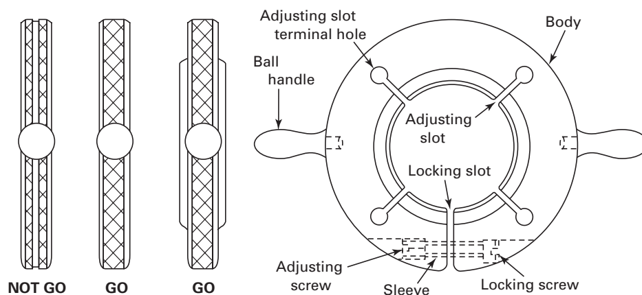
(c) Range – Above 8.510 in. to and Including 12.260 in.
