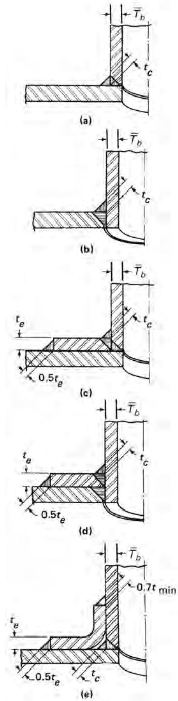
Fig. 527.3.5-4 Some Acceptable Types of Welded Branch Attachment Details Showing Minimum Acceptable Welds
