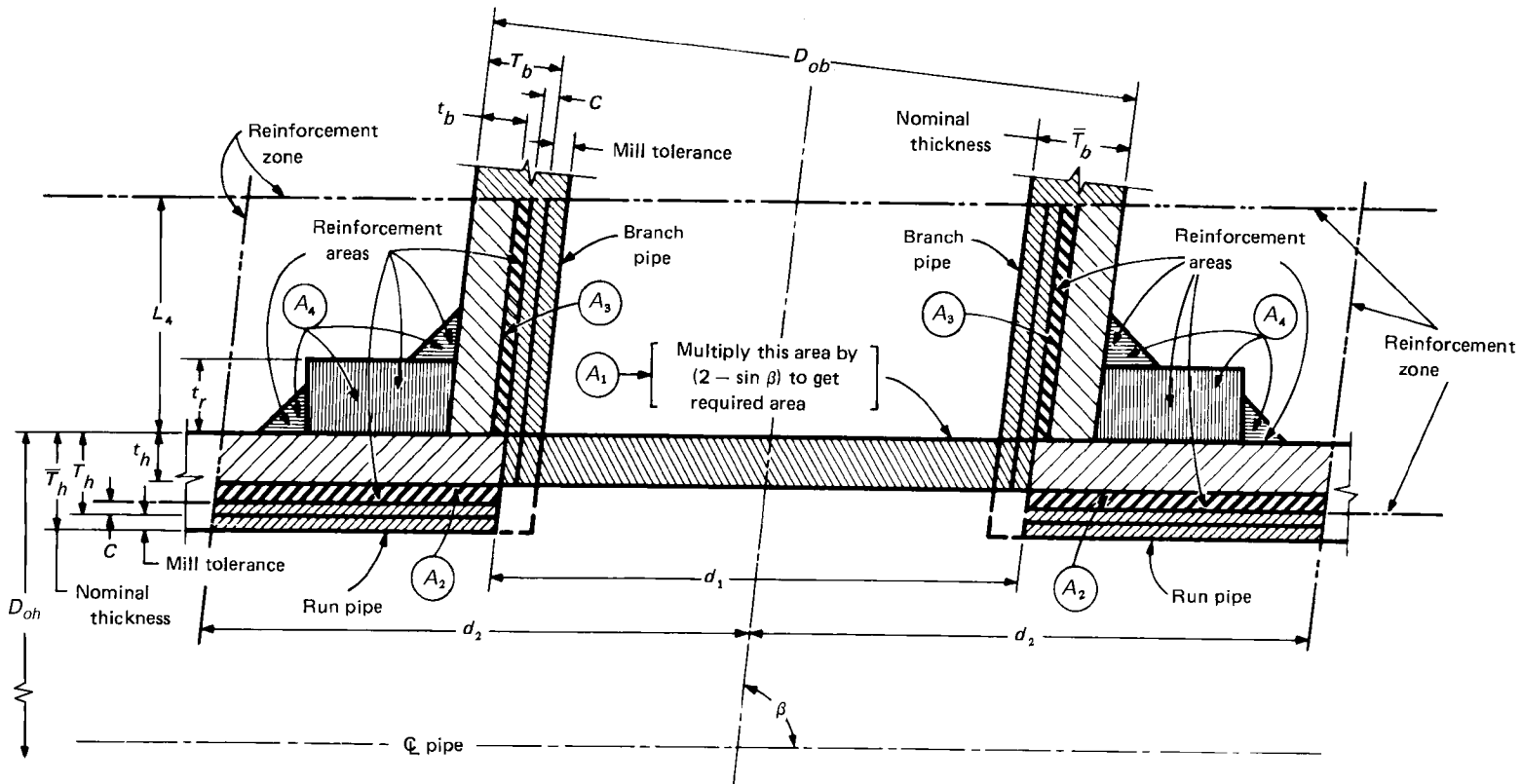
Fig. 504.3.1-1 Reinforcement of Branch Connections
