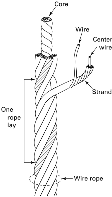
Fig. 9-2.0-2 Wire Rope
