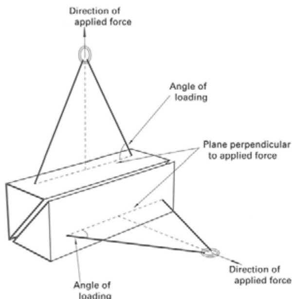
Fig. 9-6.5-1 Angle of Loading
