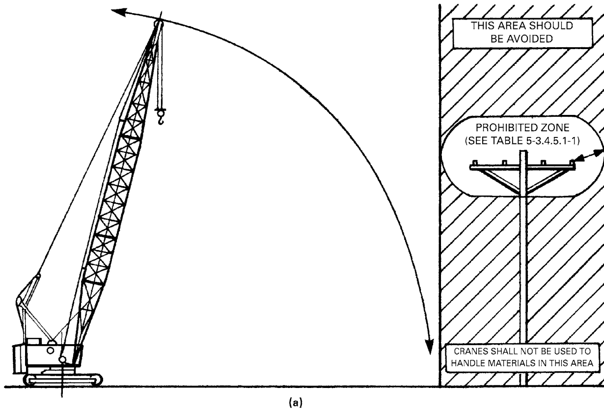
Fig. 5-3.4.5.1-1 Danger Zone for Cranes and Lifted Loads Operating Near Electrical Transmission Lines
