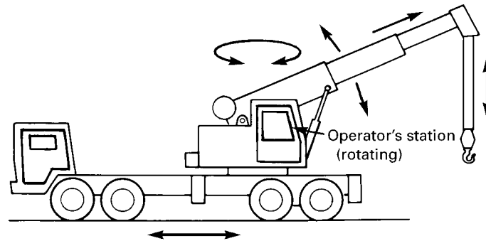
Fig. 5-0.2.1-7 Wheel-Mounted Crane — Telescoping Boom (Multiple Control Stations)
