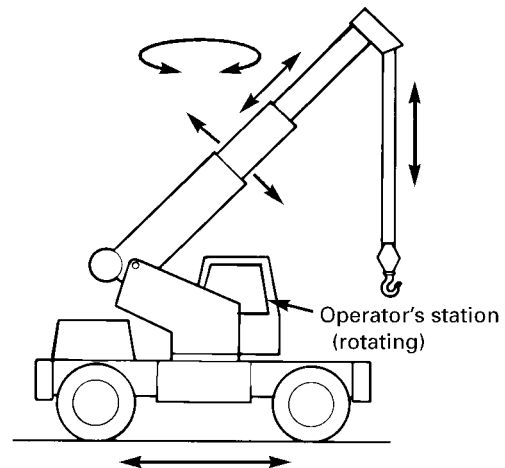
Fig. 5-0.2.1-9 Wheel-Mounted Crane — Telescoping Boom (Single Control Station, Rotating)
