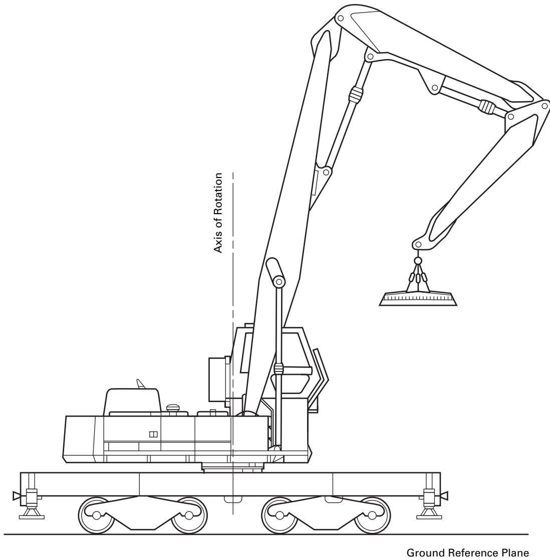
Fig. 25-0.2.1-3 Rail-Mounted Handler
