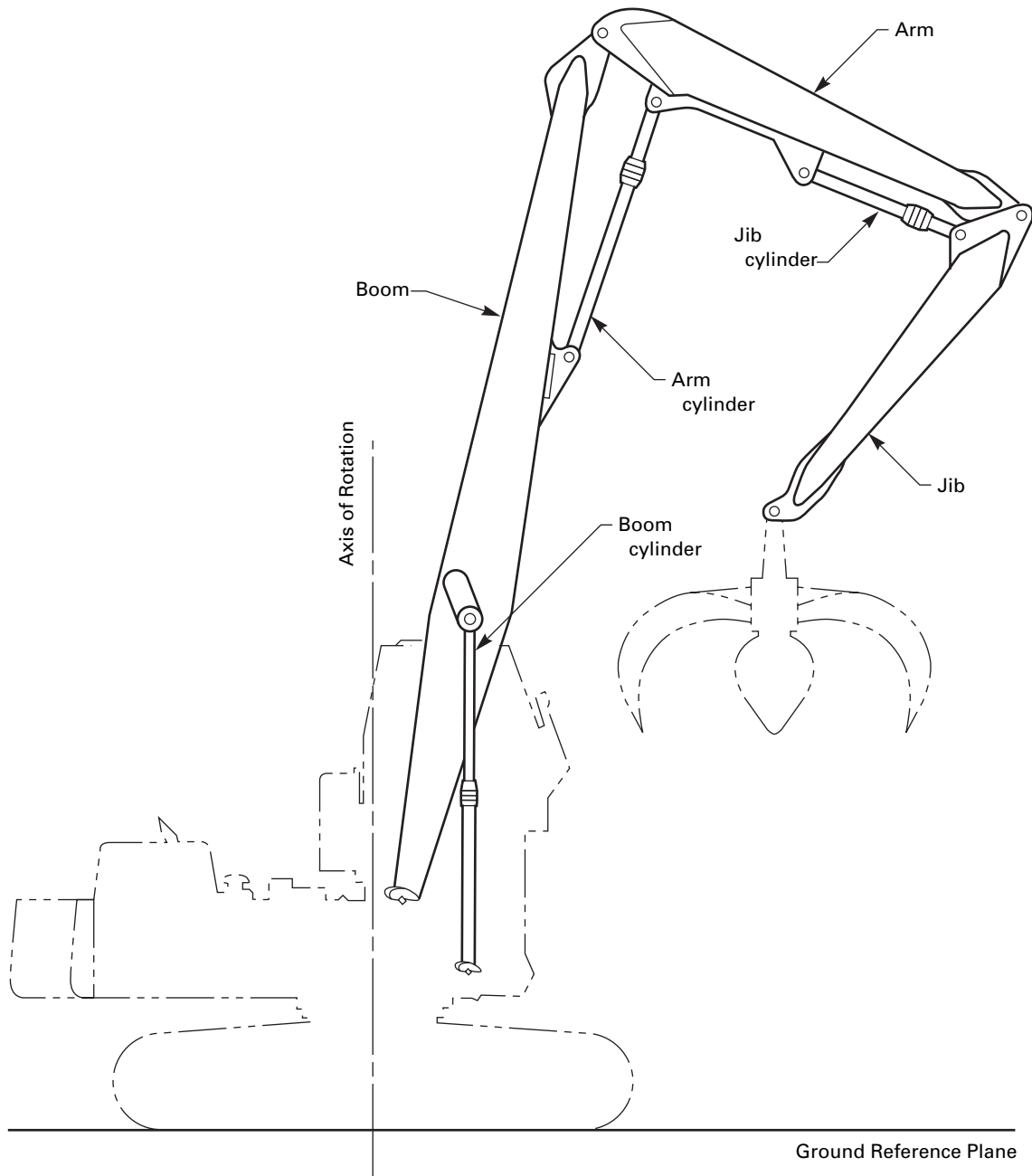
Fig. 25-0.2.2-2 Three-Piece Front
