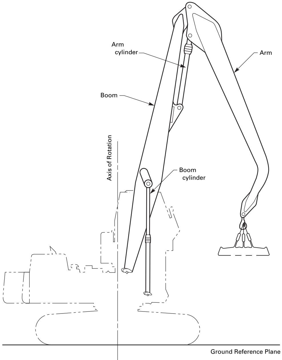
Fig. 25-0.2.2-1 Two-Piece Front
