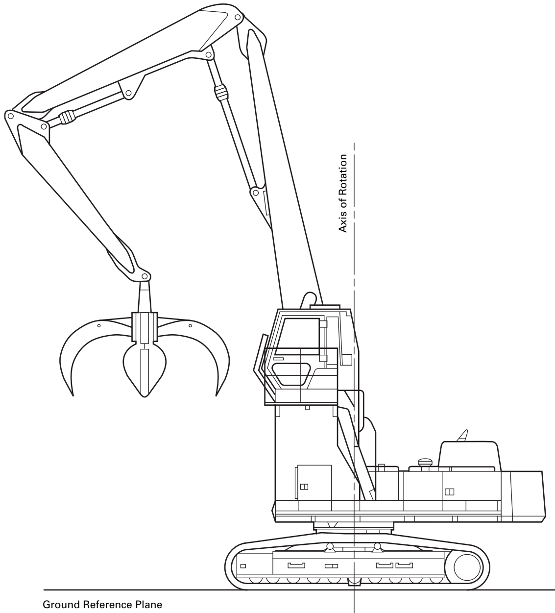
Fig. 25-0.2.1-1 Crawler-Mounted Handler
