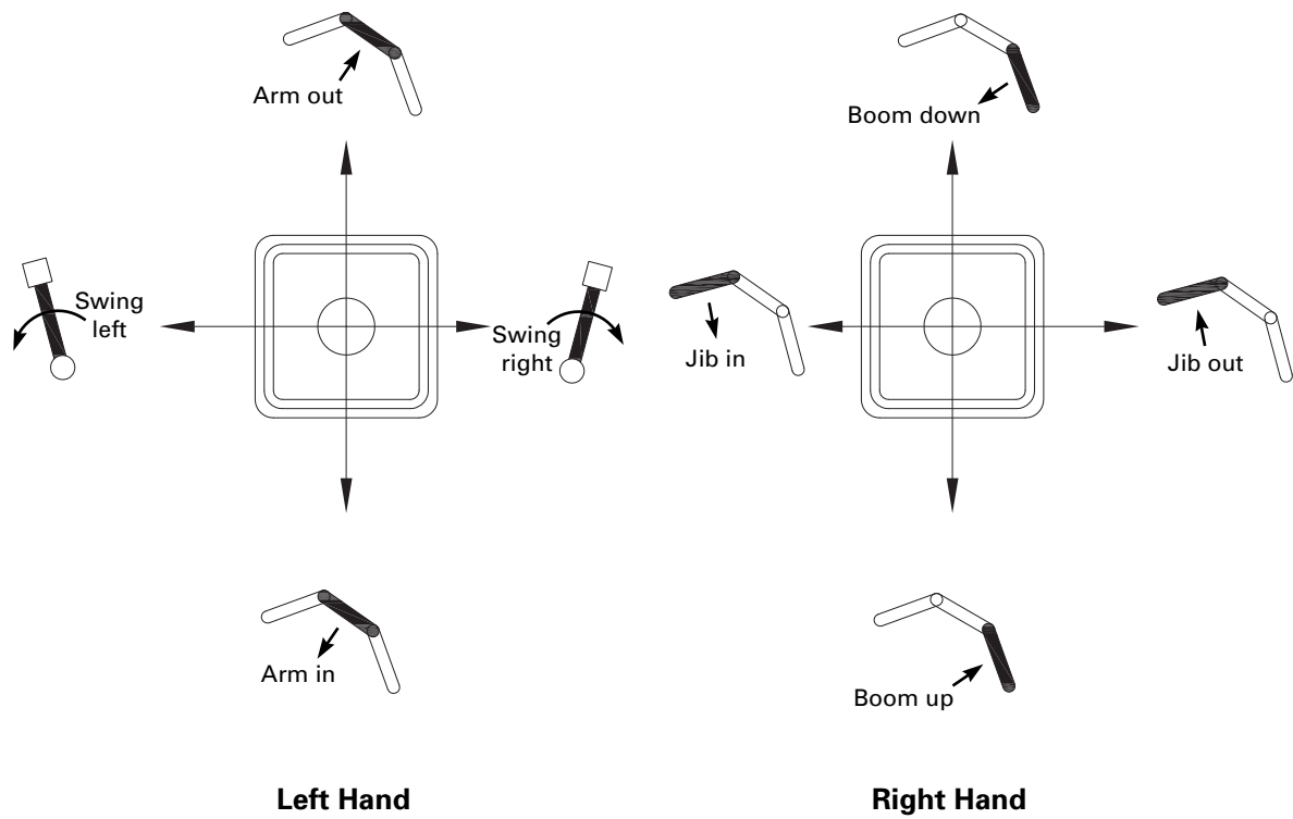
Fig. 25-1.5.3(c)-1 Primary Front Controls — Three-Piece Fronts
