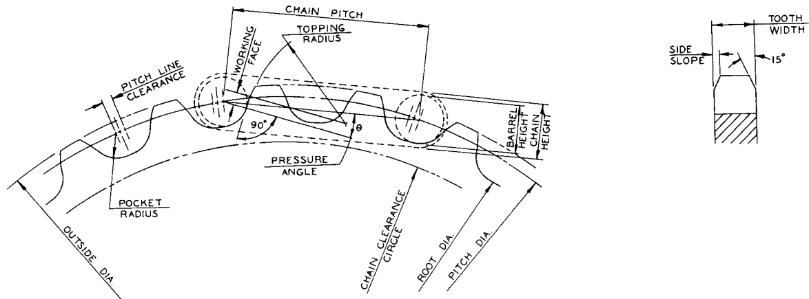
FIG. 5 SPROCKET TOOTH FORM
