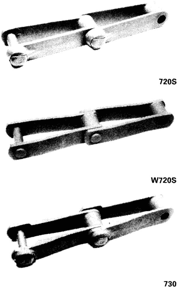
FIG. 1 STRAIGHT SIDEBAR TYPE
