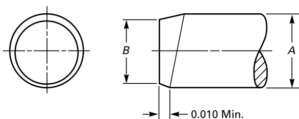
FIG. 1 POINT CONCENTRICITY
