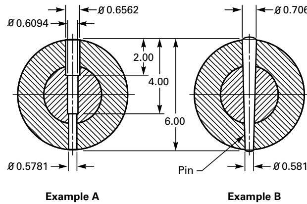
FIG. A1 DRILL DIAMETER EXAMPLES
