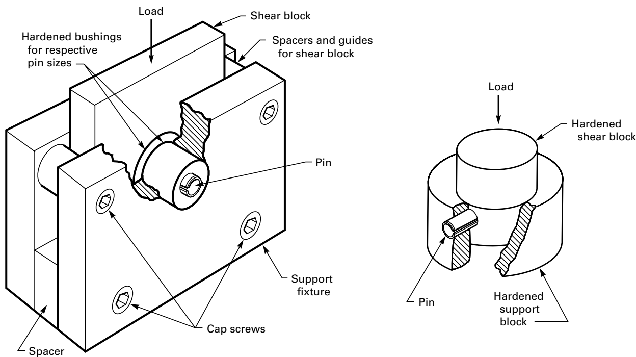
FIG. B1 TYPICAL PIN SHEAR TEST FIXTURES
