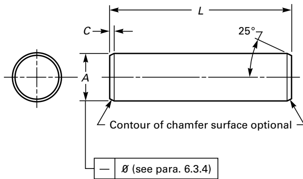
Chamfered Straight Pin
