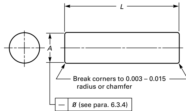
Square End Straight Pin
