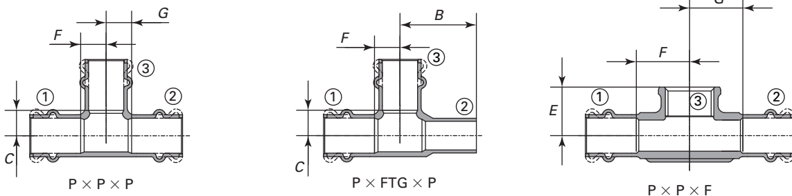
(h) Tees
