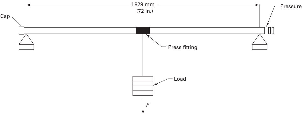
Fig. 6 Test Setup for Bending Test
