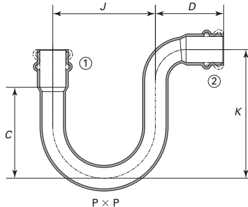
(j) Suction Line P-Traps
