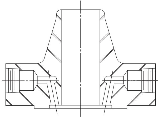
Fig. 1 Corner Taps
