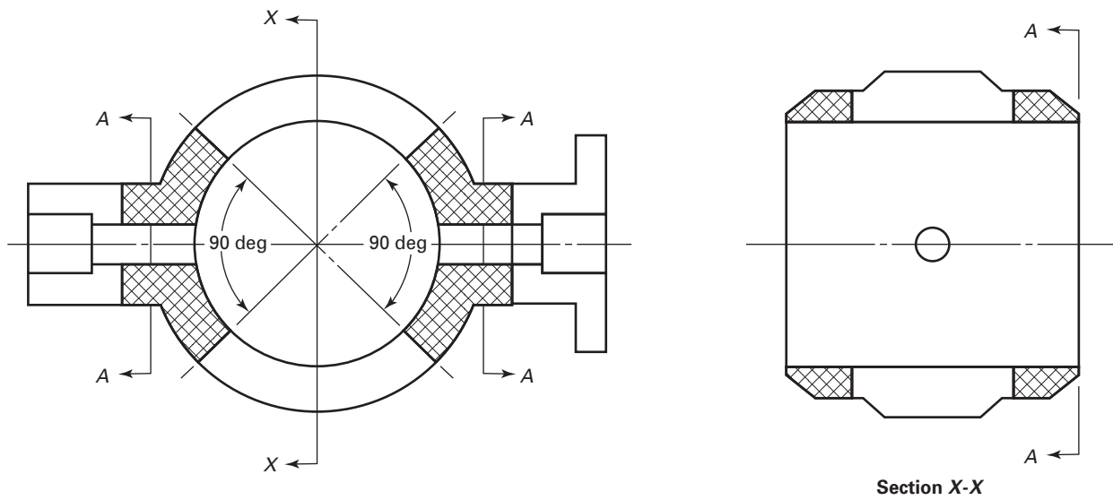
Fig. 13 Butterfly Body
