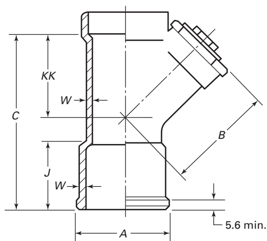
DWV 45-deg Y With Cleanout
