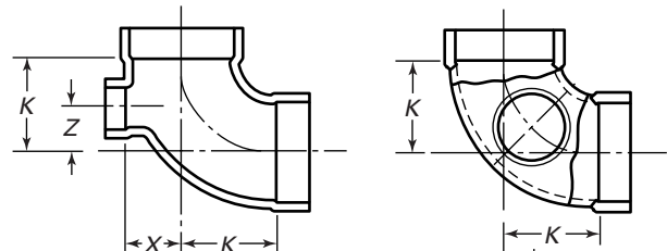
DWV 90-deg Elbow With High Heel Inlet C × C × C
