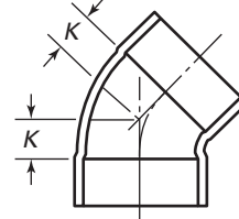
DWV 45-deg Elbow C × C
