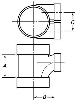
DWV Horizontal Twin Branch Tees C \times C \times C \times C
