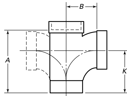
DWV Fitting Tees — Single and Double FTG \times C \times C FTG \times C \times C \times C
