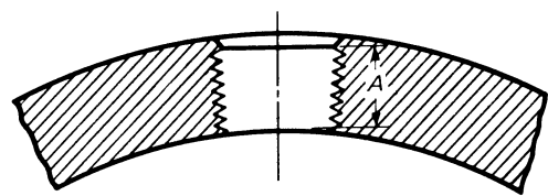
Fig. 2 Drain Connections
