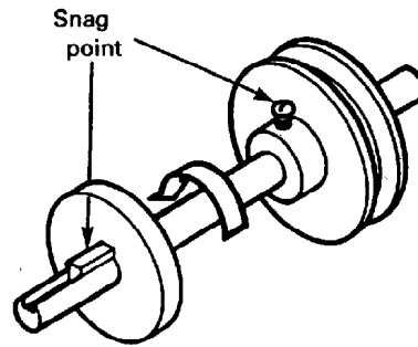
FIG. 8 ROTATING MOTION
