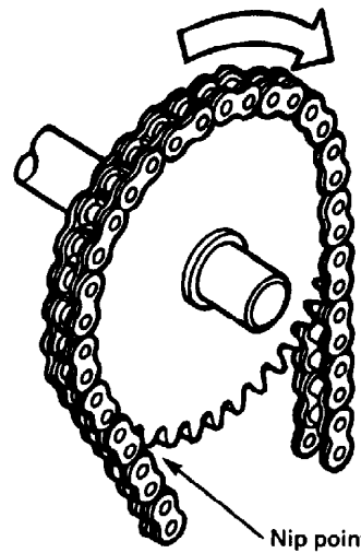
FIG. 2 ROTATING MOTION
