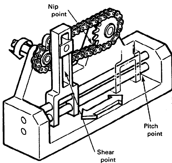
FIG. 11 ROTATING / RECIPROCATING MOTION
