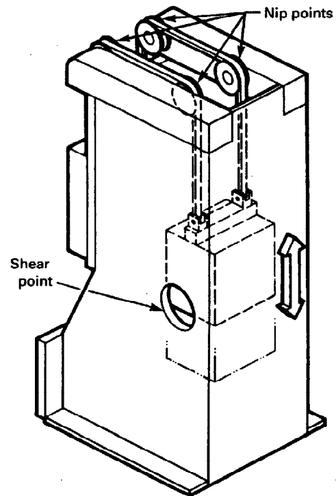
FIG. 10 ROTATING / RECIPROCATING MOTION
