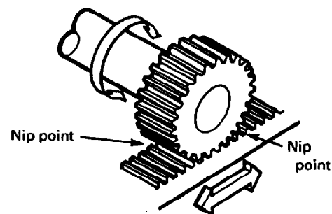
FIG. 4 ROTATING / RECIPROCATING MOTION
