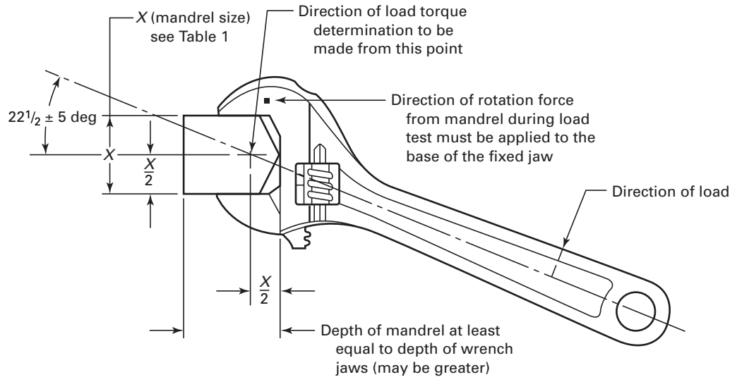
Fig. 2 Test Configuration
