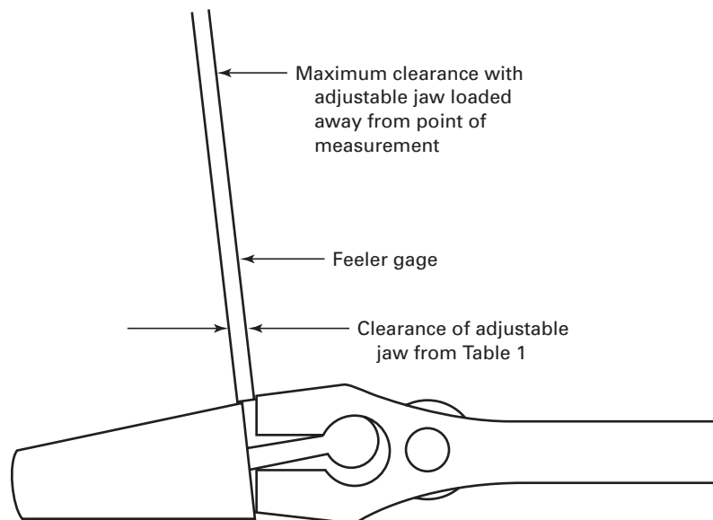
Fig. 3 Jaw Clearance Measurement
