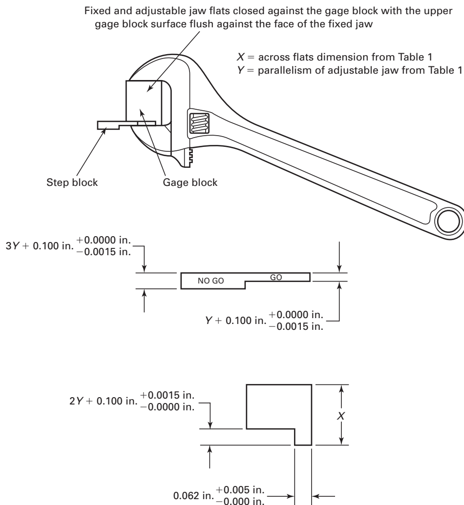
Fig. 5 Parallelism Measurement
