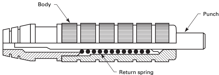
Fig. 2 Type II (Self-Centering) Nail Set
