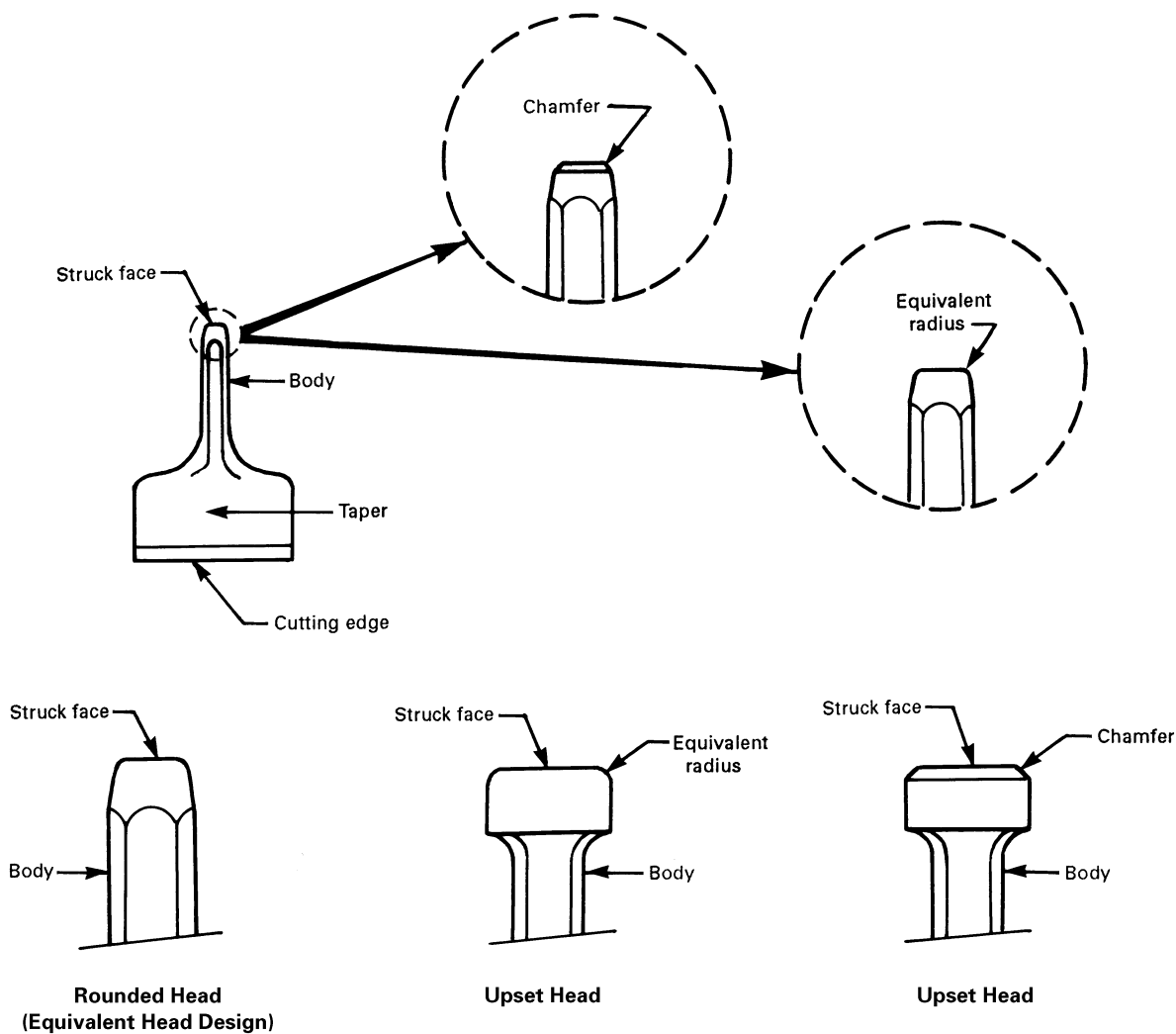
Fig. 1 Nomenclature for Brick Chisel and Brick Set
