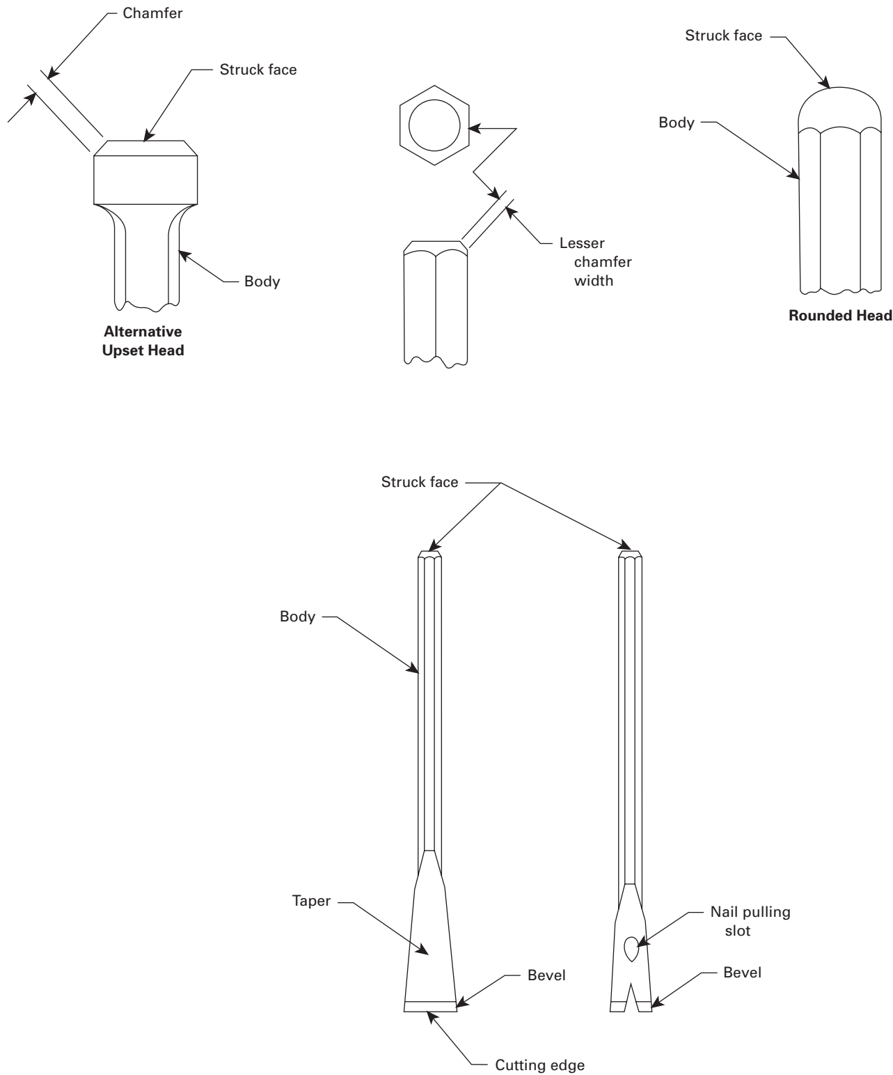
Fig. 4 Nomenclature for Ripping Chisels
