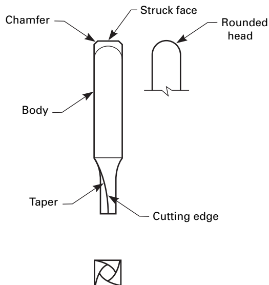
Fig. 3 Nomenclature for Spiral Flute Extractor
