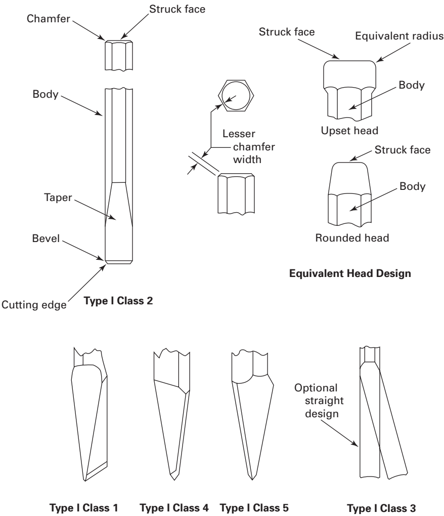
Fig. 2 Nomenclature for Type I Chisels
