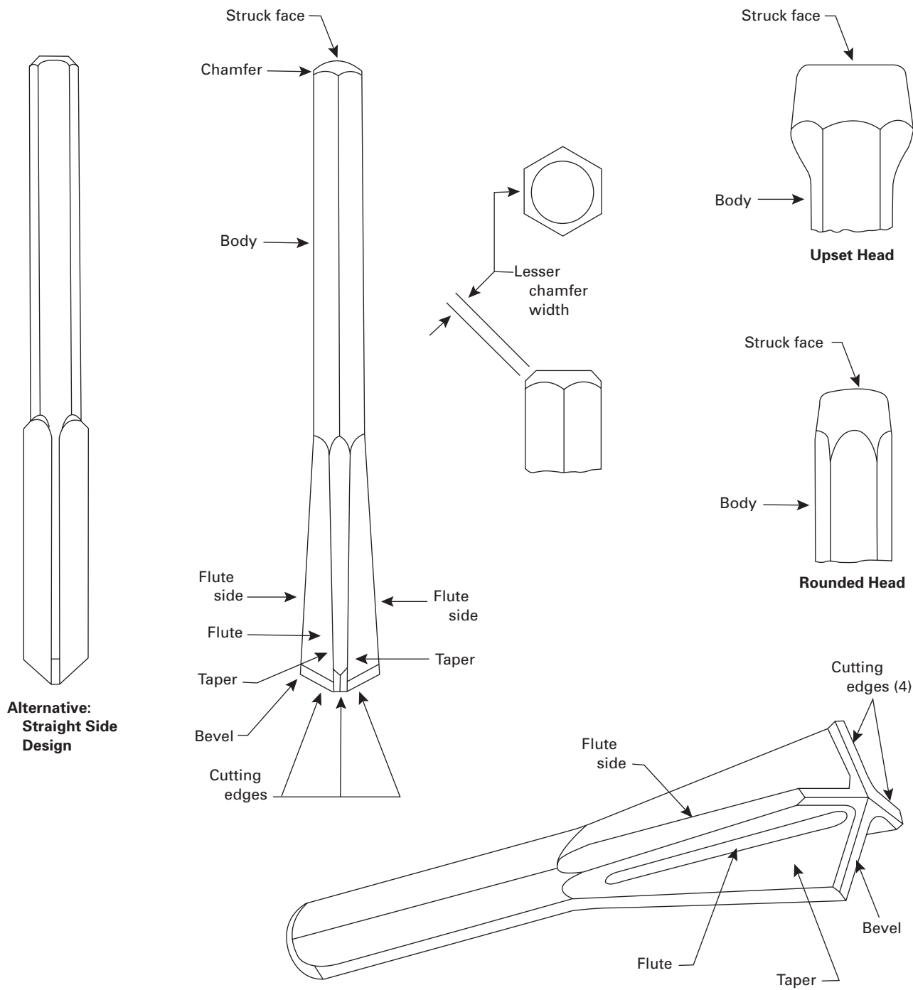
Fig. 3 Nomenclature for Star Drill
