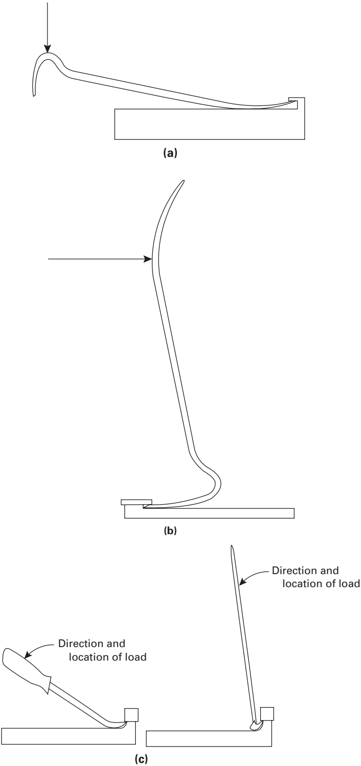
Fig. 9 Prying Test
