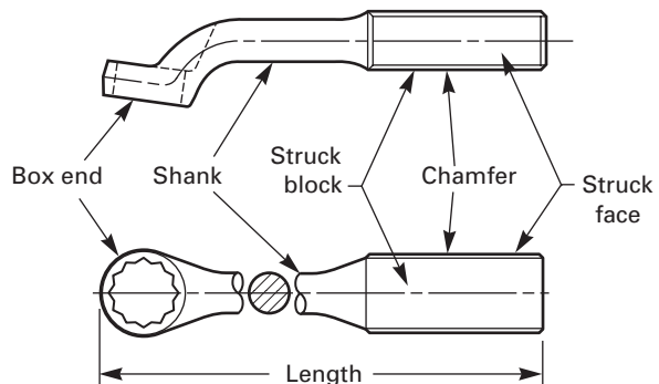
Fig. 1 Nomenclature for Striking Wrenches
