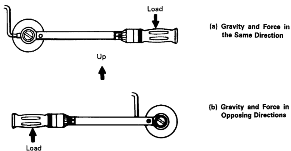
FIG. 14 GRAVITY DEPENDENT TESTING POSITION
