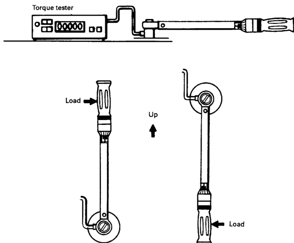
FIG. 13 GRAVITY INDEPENDENT TESTING POSITION — GRAVITY AND FORCE AT 90 DEG. TO EACH OTHER
