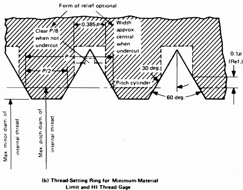
FIG. 8 THREAD FORM OF SOLID THREAD-SETTING RING GAGES
