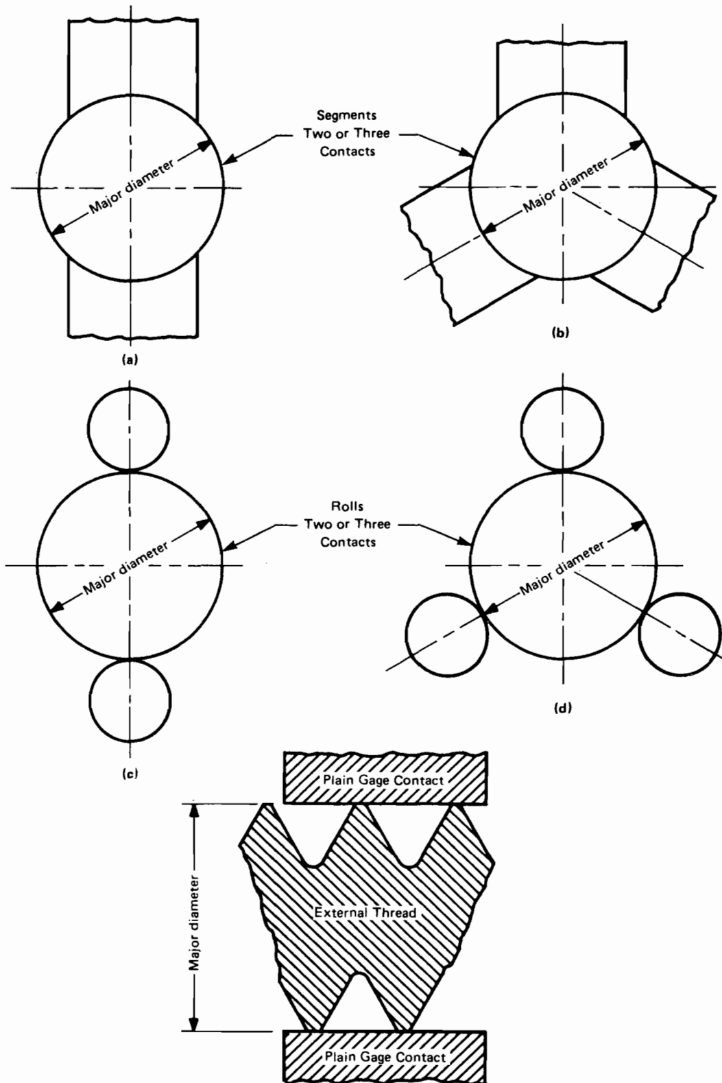
FIG. 33 INDICATING PLAIN DIAMETER GAGE — MAX.-MIN. MAJOR DIAMETER LIMIT AND SIZE
