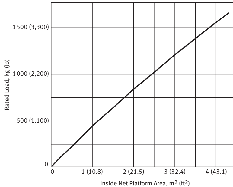
Fig. 9.7 Minimum Loads to Sustain and Lower Based Upon Inside Net Platform Area
