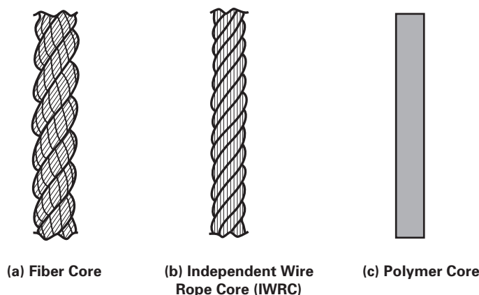
Fig. 1.3.1.4-1 Examples of Cores
