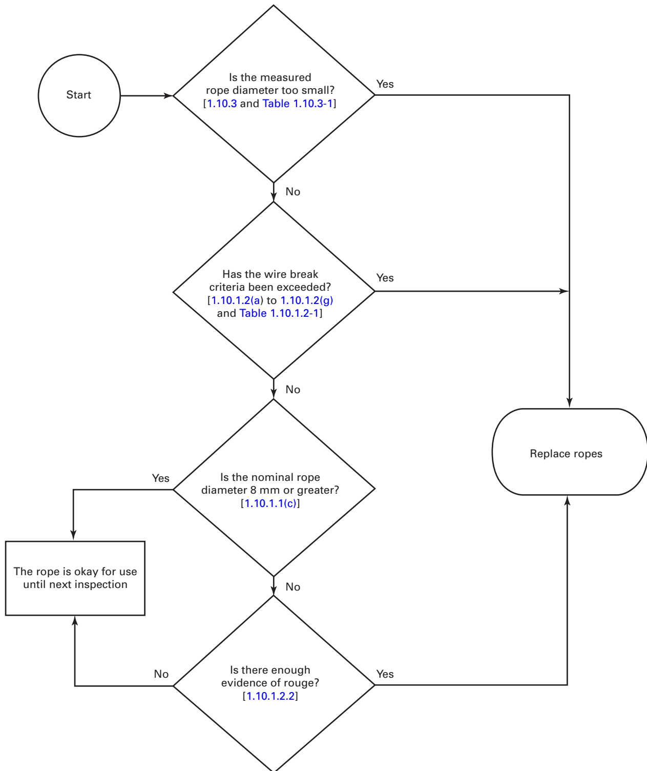
Fig. A-1 Inspection and Replacement of Steel Wire Ropes
