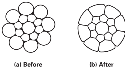
Fig. 1.3.1.3.2-2 Compacted Round Strand: Before and After Compacting
