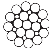
Fig. 1.3.1.3.4-3 Filler Construction (e.g., 25F, 12-6F-6-1)
