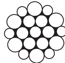
Fig. 1.3.1.3.4-2 Warrington Construction [e.g., 19W, (6+6)-6-1]
