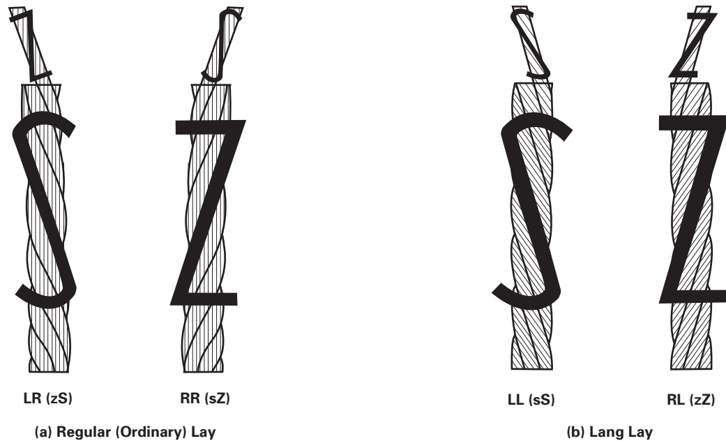
Fig. 1.3.2.4.2-1 Regular (Ordinary) Lay and Lang Lay
