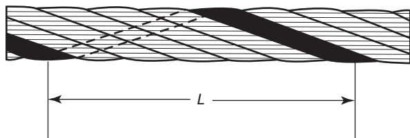
Fig. 1.3.3.2.2-1 Rope Lay Length
