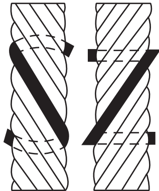
Fig. 1.3.1.3.3-1 Lay Direction of Strands for Stranded Ropes
