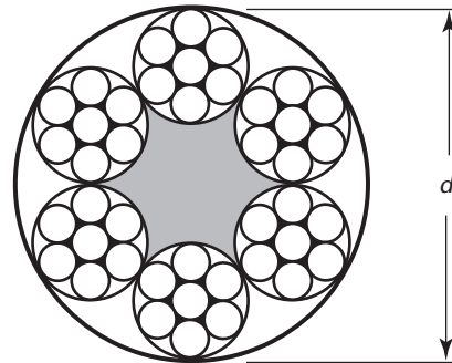
Fig. 1.3.3.1.1-1 Diameter of Round Rope
