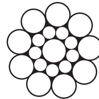
Fig. 1.3.1.3.4-1 Seale Construction (e.g., 19S, 9-9-1)
