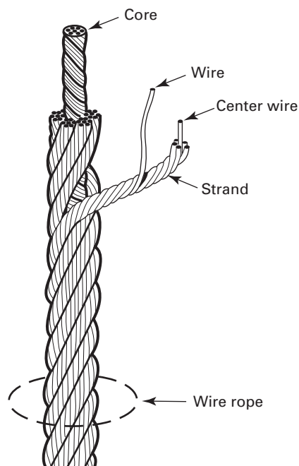
Fig. 1.3.1.1-1 Elements of Stranded Steel Wire Rope
