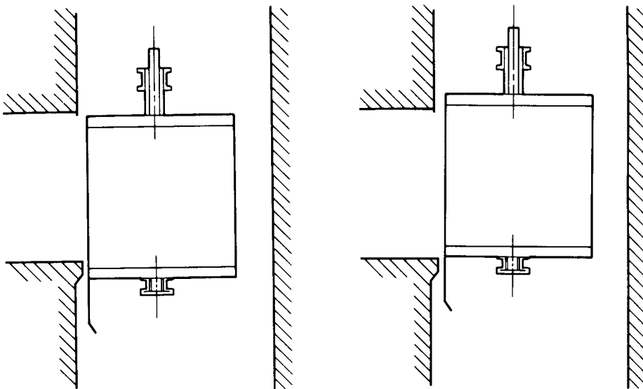
Fig. 1.3.3 Car at or Near Landing
