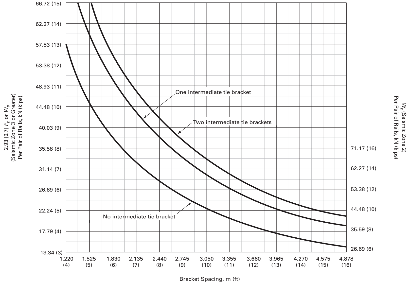
Fig. 8.4.8.2-1 12 kg/m (8 lb/ft) Guide-Rail Bracket Spacing
