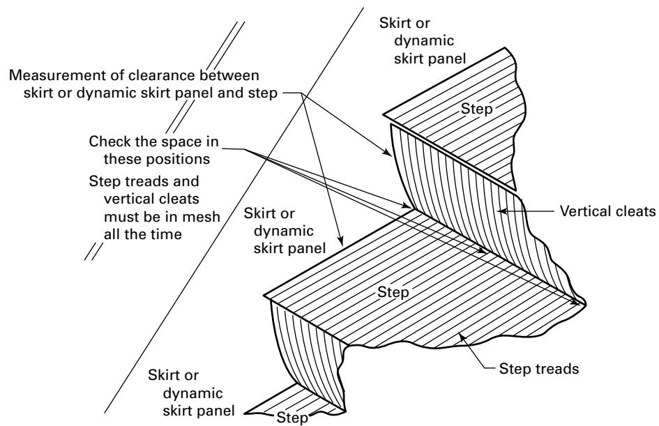
Fig. I-8 Cleated Riser (6.1.3.5.3)
