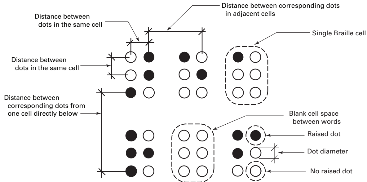
Fig. E-20.4 Braille Measurements
