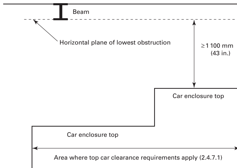
Fig. G-2 Additional Top-of-Car Clearance Requirements (2.4.7.1)
