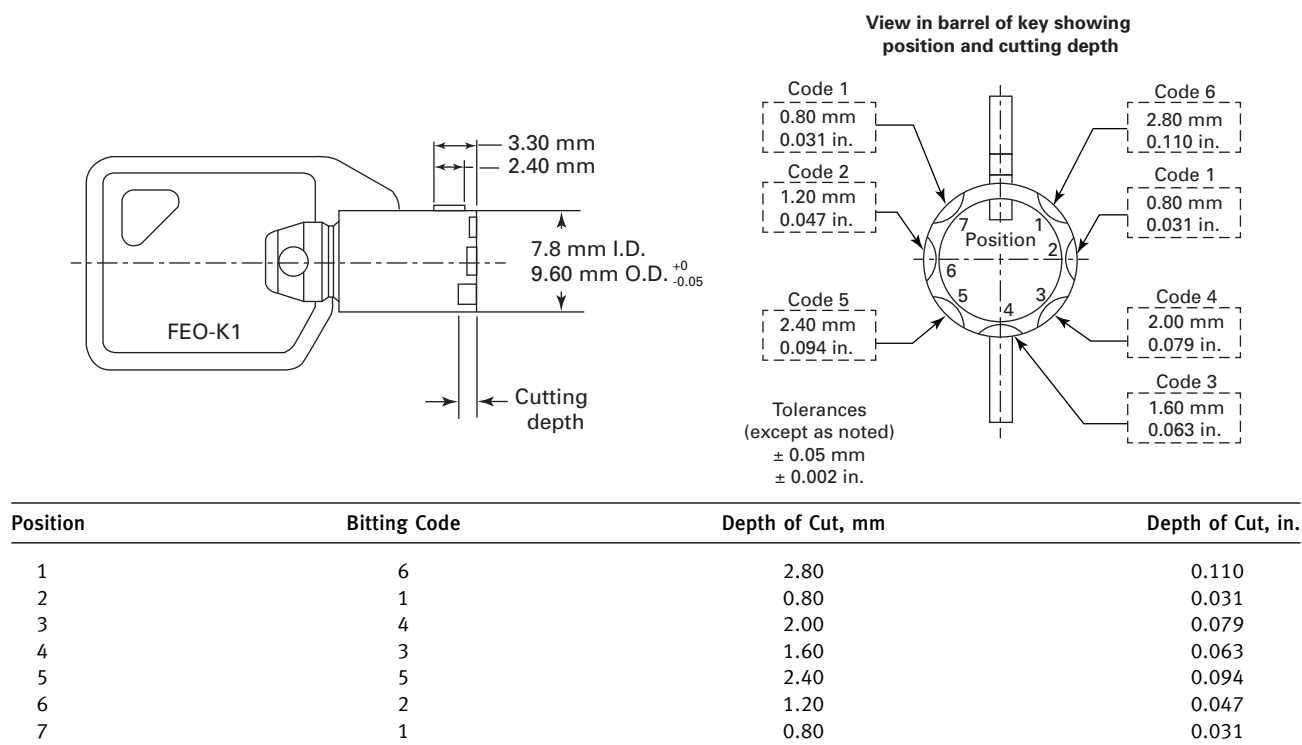
Fig. 2.27.8 FEO-K1 Key
