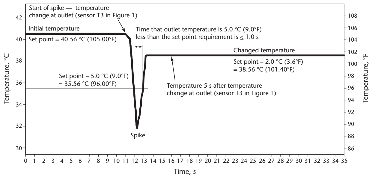
Figure B.2 Example of temperature decrease spike (See Sections 4.6.2 and 4.6.8.)
