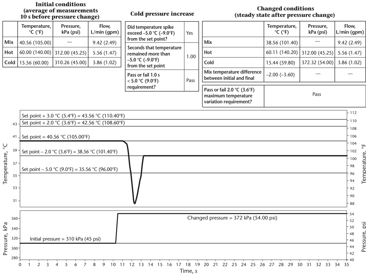
Figure B.5 Example of temperature record for temperature decrease spike (See Section 4.6.2. )
