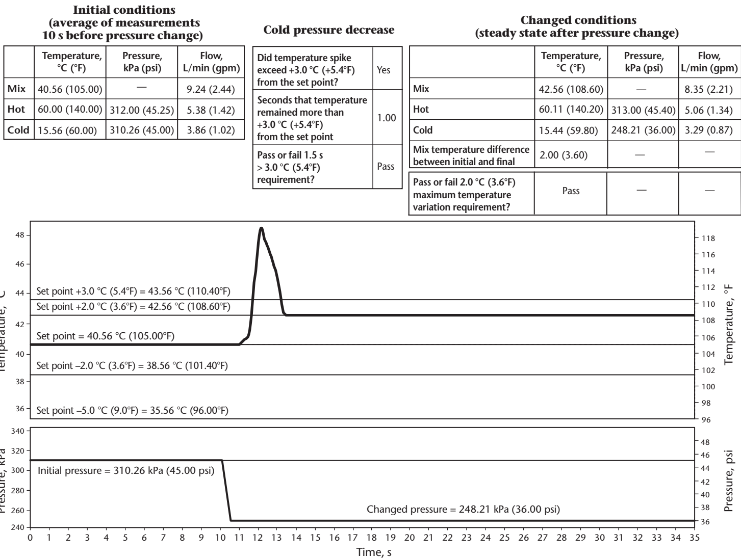
Figure B.4 Example of temperature record for temperature increase spike (See Section 4.6.2. )
