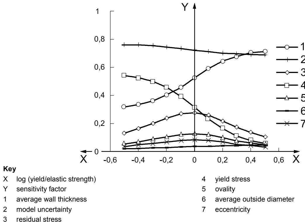
Figure F.15 — Sensitivity factors
