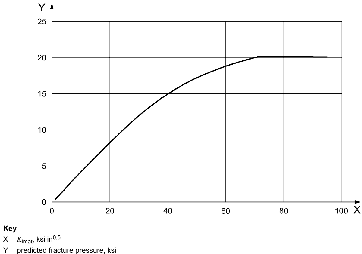
Figure D.1 — Influence of K_{\text{Imat}} on fracture propagation pressure (7 in diameter, 0.730 in wall, C90 with 5 % imperfection, 0.875 wall factor)
