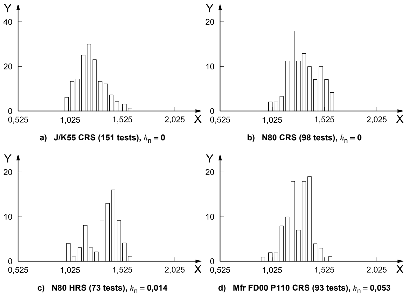
Figure F.12 — Comparison of design collapse strengths with collapse test data (sharp-kneed SSCs), h_n = 0
