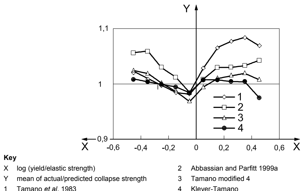
Figure F.1 — Predictive accuracy (mean) vs. dataspace position
