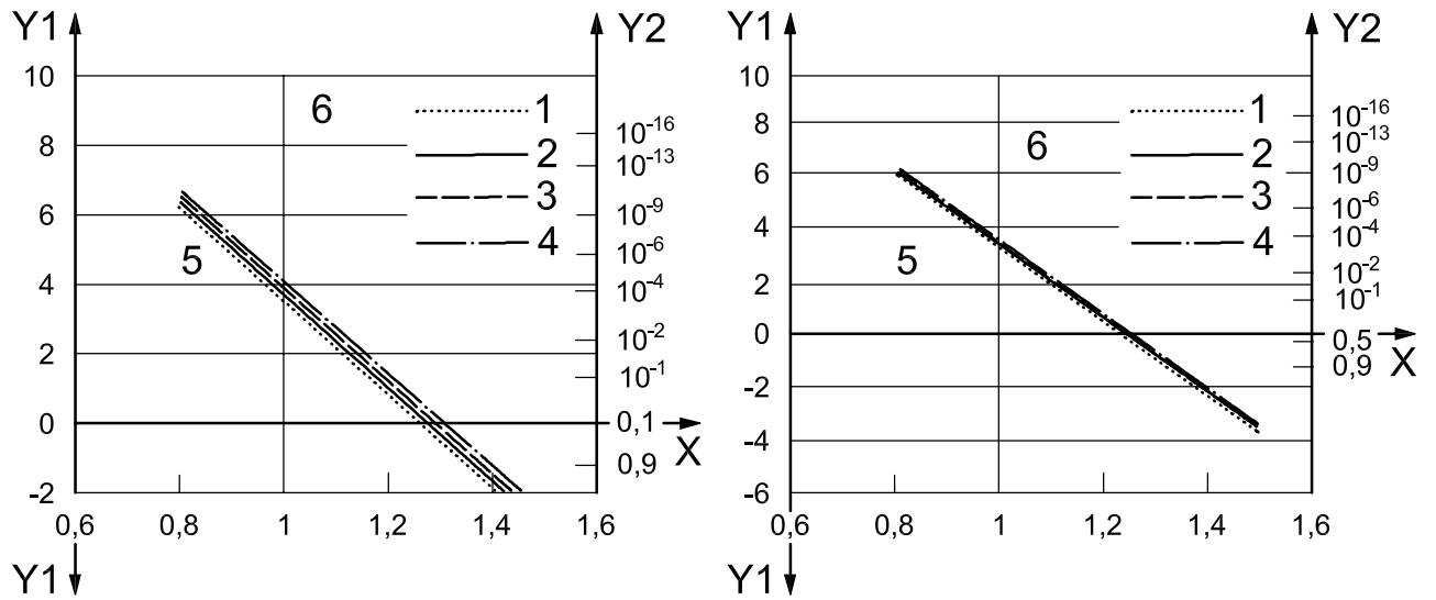
a) Single joint — Mean factor of safety of 1,3
