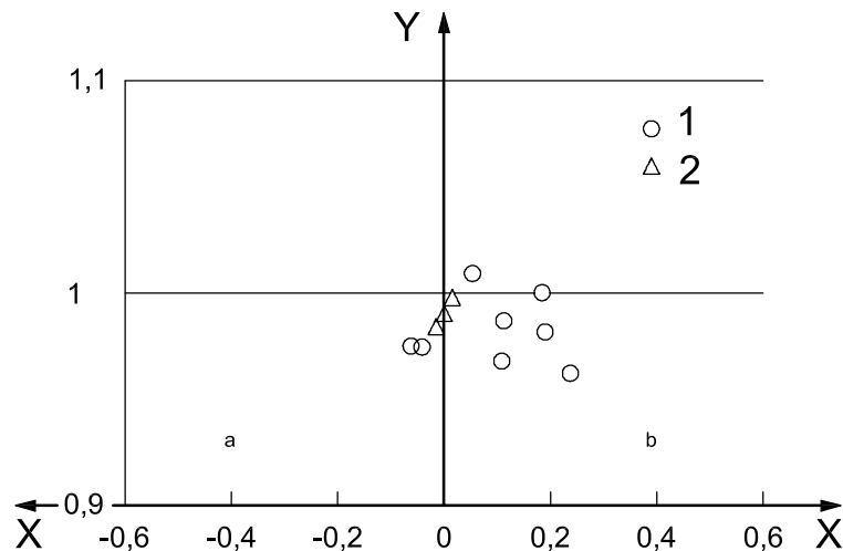
Figure F.2 — Actual/Klever-Tamano predicted strength vs. dataspace position
