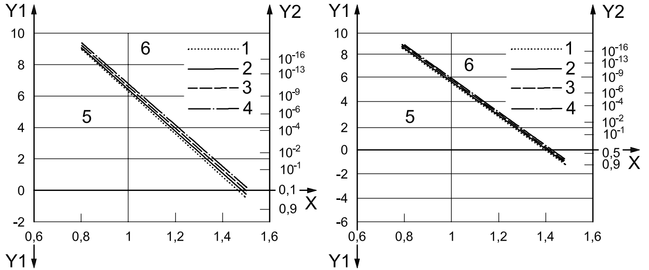
b) Deepest defect in 50 joints — Mean factor of safety of 1,3
