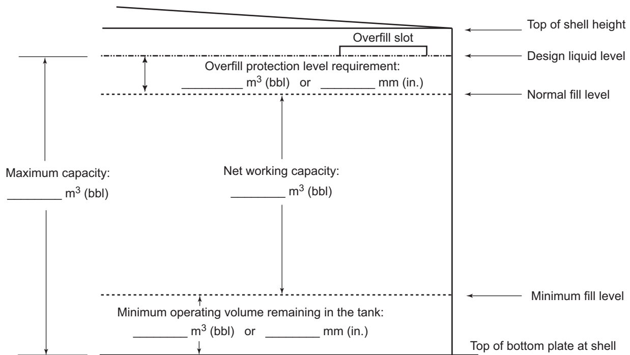
Figure 5.4—Storage Tank
