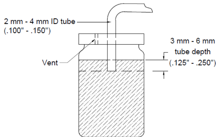
Figure 1—Volumetric Device
