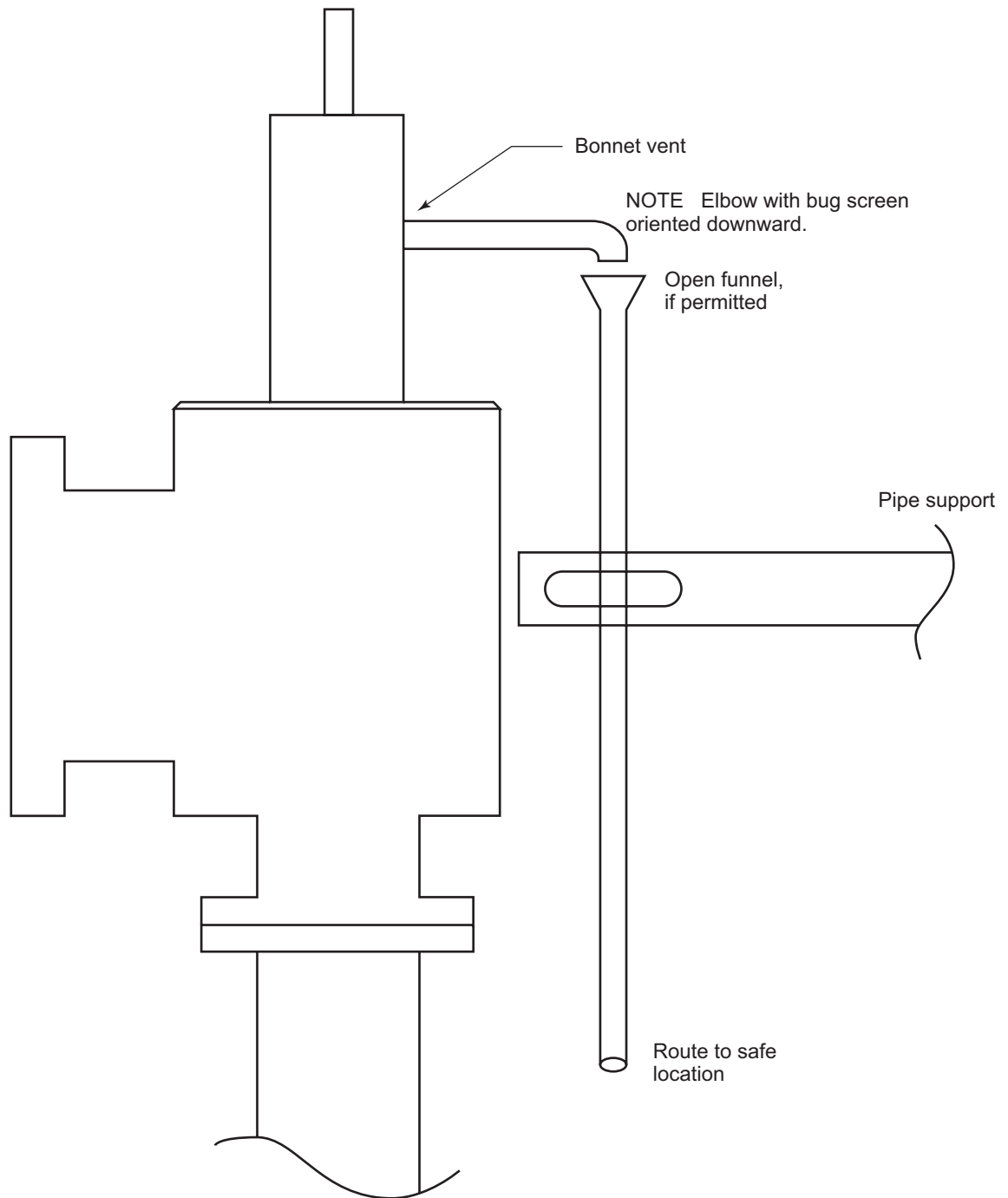
Figure 22—Bonnet Vent for Bellows Valves Handling Liquids Where a Leak Needs to Be Routed Away from the PRV
