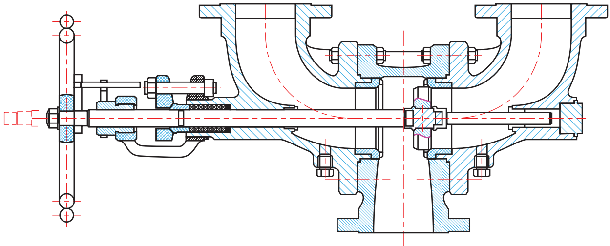
Figure 14—Three-Way Changeover Valve—Shuttle Type
