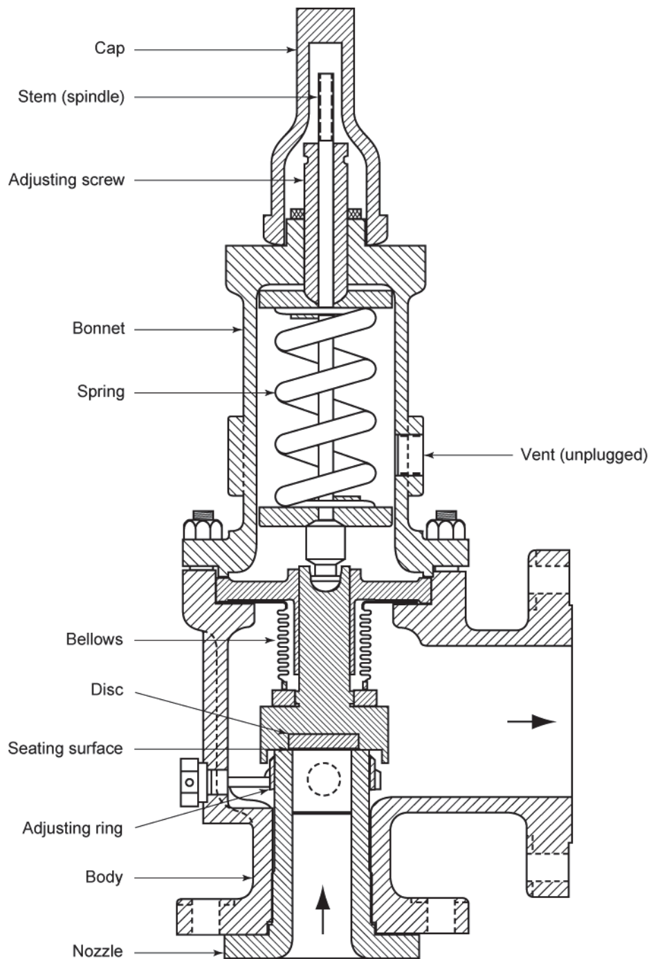
Figure 2—Balanced-bellows PRV
