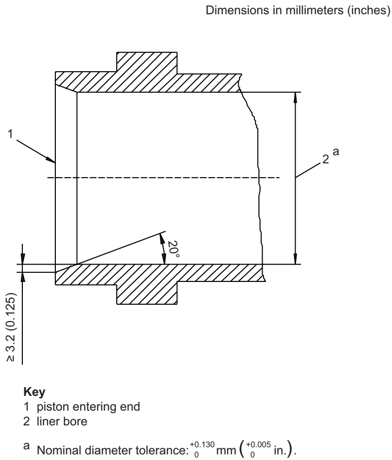
Figure 22—Mud-pump Liner
