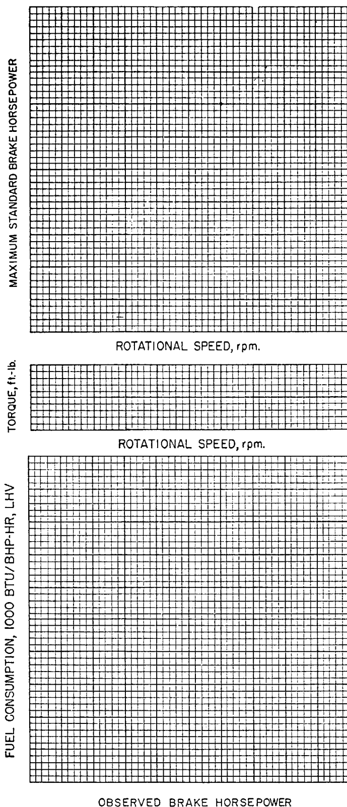
Figure 2—Test Report Form for Internal-Combustion Power Units (Continued) (See Figure 4 for examples of test-data curves)
