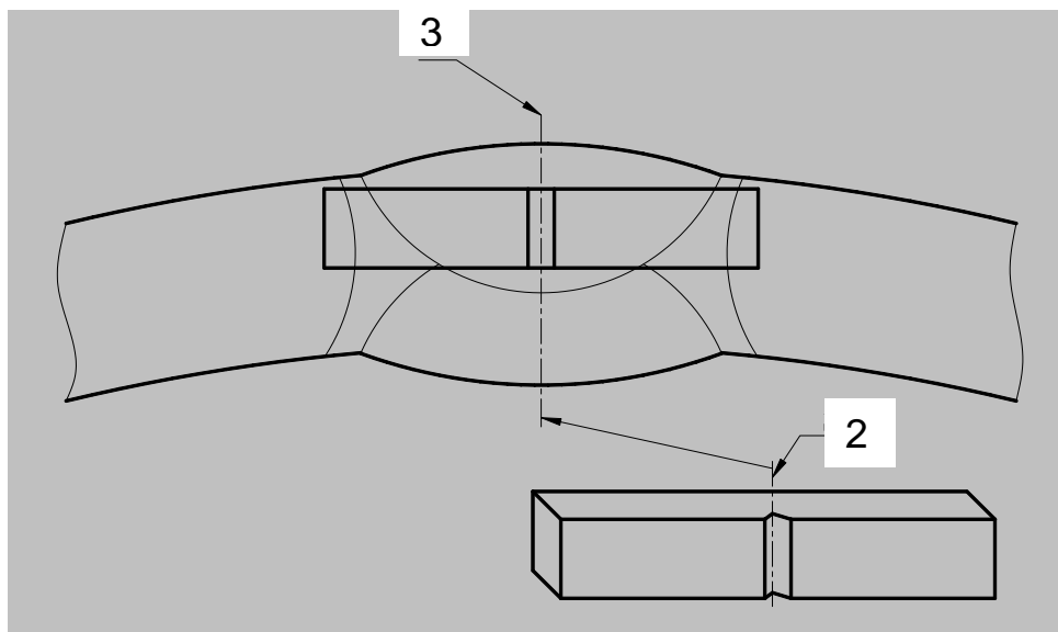
b) Weld specimen
